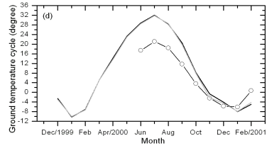
Fig 6 Diurnal and seasonal energy cycle (Units: Wm^{-2} ) and air surface temperature (Units: Degree) at Dunhuang Gobi. (b) Ground temperature diurnal cycle (d) Ground temperature seasonal cycle. Marks 'TG' means ground temperature; 'OBS' mean the observations, others on the panels have the same meanings with Fig 4
