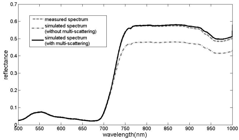
Fig. 1. Figure 3. Impacts of multi-scattering on reflectance spectra
