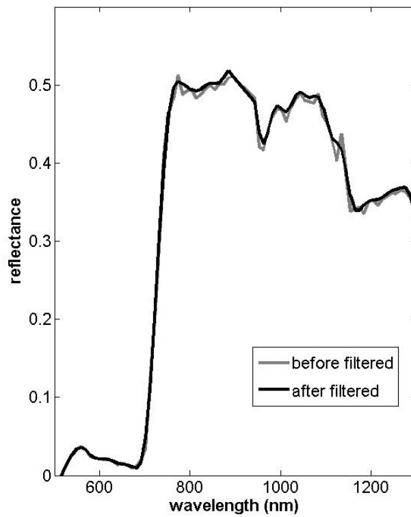
Fig. 3. Fig. 7 Hyperion spectrum before and after filtered by using the innovative filtering method
