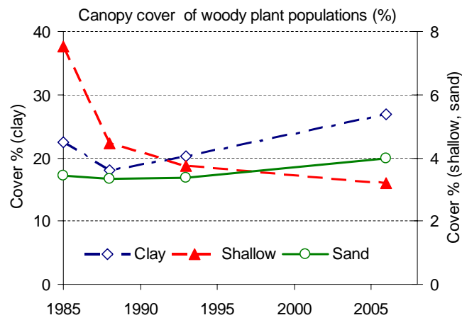
Changes of the mean the canopy cover of woody populations over low-land clay soils (5 sites, left scale), dunes and low-land sandy soils (13 sites, right scale) and eroded slopes shallow soils (4 sites, right scale) in the Gourma following the 1983-84 drought (adapted from Hiernaux et al. 2009a).
