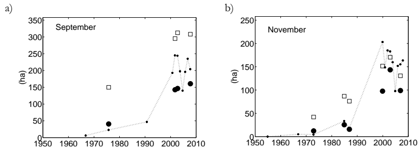
a) Average surface of water per pond (open square), average surface of turbid water (full circle) for the 91 ponds present in all September Landsat images. Also figured is the surface of the Agoufou pond in September (line), derived from all data sources. b) same as (a) but for November and for the 51 ponds present in all November Landsat images.
