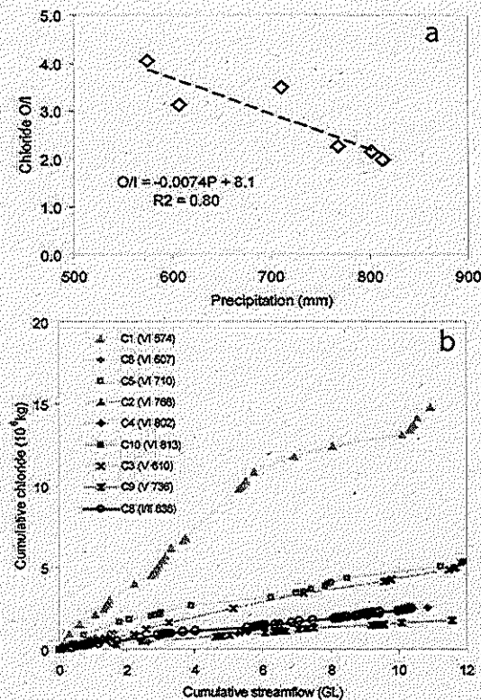
Fig. 7. (a) Catchment chloride ratio vs. catchment average annual precipitation for six type VI catchments, indicating that a catchment of an average precipitation of 960 mm would have now (2008) reached the new chloride equilibrium (type II). (b) Cumulative chloride load in the stream water vs. cumulative streamflow for six type VI catchments, showing that the average chloride concentration (the slope of the curve) decreases with increasing annual precipitation (the number in the legend), with two type V catchments and one chloride equilibrium catchment for comparison.
