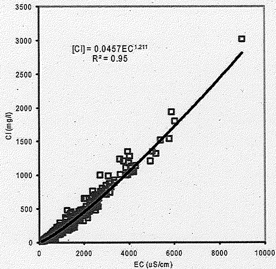
Fig. 3. Measured chloride concentration of stream water vs. measured electrical conductivity values, based on 306 samples by EPA mainly collected in May and October, and 145 samples by DWLBC collected in November, December, March, and July.
