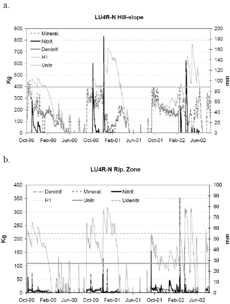
Figure 8. Simulated soil moisture content ( H_1 ), nitrification soil moisture threshold ( U_{\text{nitr}} ) and denitrification soil moisture threshold ( U_{\text{denitr}} ) in mm, plus simulated mineralization, nitrification and denitrification processes (kg) for the riparian zone (calibration period 1999-2002) with the LU4R-N model
