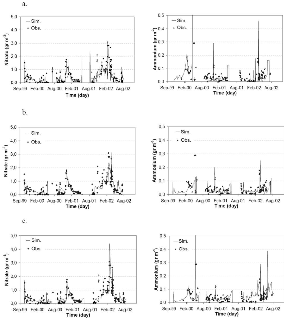
Figure 4. Simulated and observed nitrate and ammonium ( \text{gr m}^{-3} ) for the calibration period (1999-2002) with a) LU4-N; b) LU4-R-N (with 2 HRUs) and c) SD4-R-N (with 4 HRUs)
