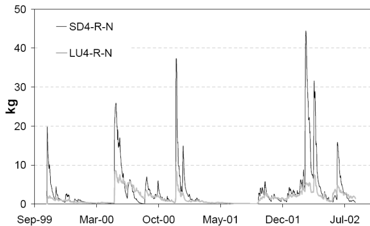
Figure 11. Simulated denitrification process (kg) in the riparian local aquifer with the LU4-R-N and SD4-R-N models.
