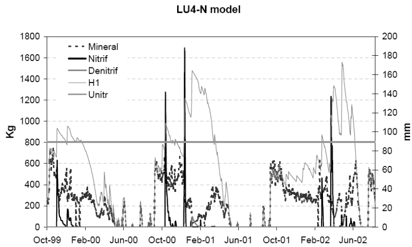
Figure 5. Simulated soil moisture content ( H_1 ) and nitrification soil moisture threshold ( U_{nitr} ) in mm, plus mineralization, nitrification and denitrification processes (kg) for the calibration period (1999-2002) with the LU4-N model
