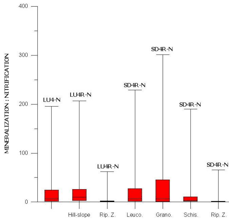
Figure 6. Simulated Mineralization:Nitrification ratio (M:N) variation according to the different models structures and to each HRU considered.
