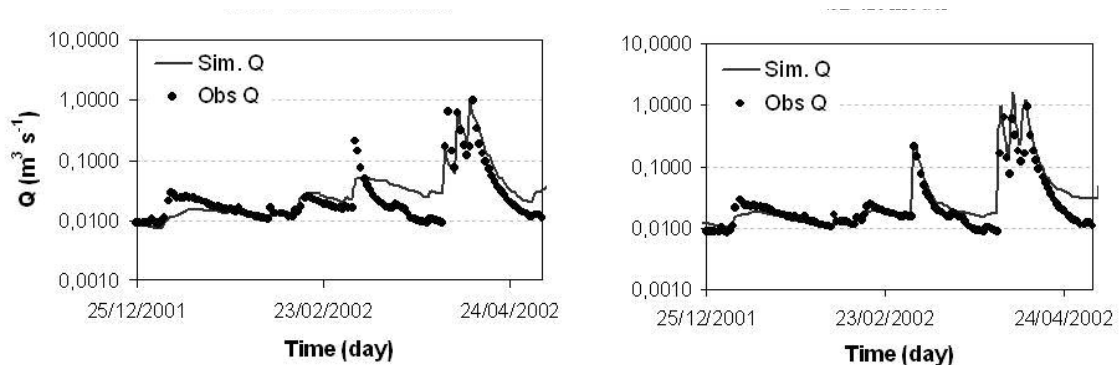
Figure 9. Simulated and observed discharges ( \text{m}^3 \text{s}^{-1} ) for the event of March 2002 obtained with: a) the LU4-R-N model and b) the SD4-R-N model.
