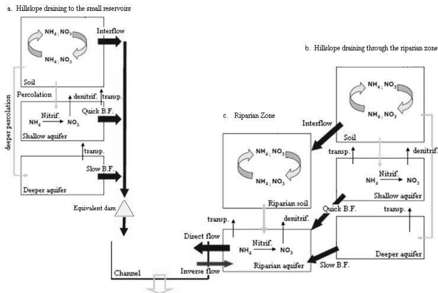
Figure 3. LU4-R-N and SD4-R-N conceptual scheme, where a) represents the part of the catchment that drains to the four small reservoirs located at the catchment; b) represents the part of the catchment that drains through the riparian zone before reaching the stream channel and finally c) represents the riparian zone which presents a bidirectional flow with the channel.
