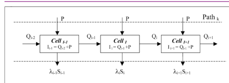
Figure 1. Runoff process and flow path.
