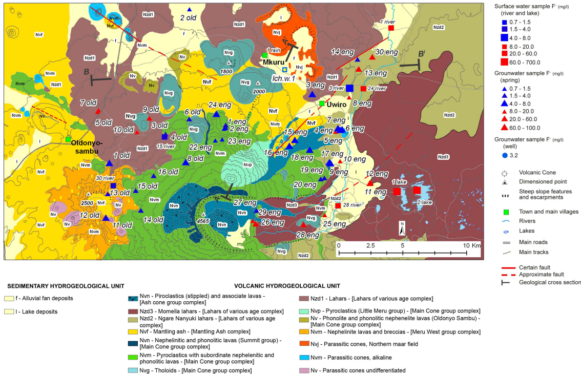
Fig. 2. Geological-Hydrogeological map with water location points.
