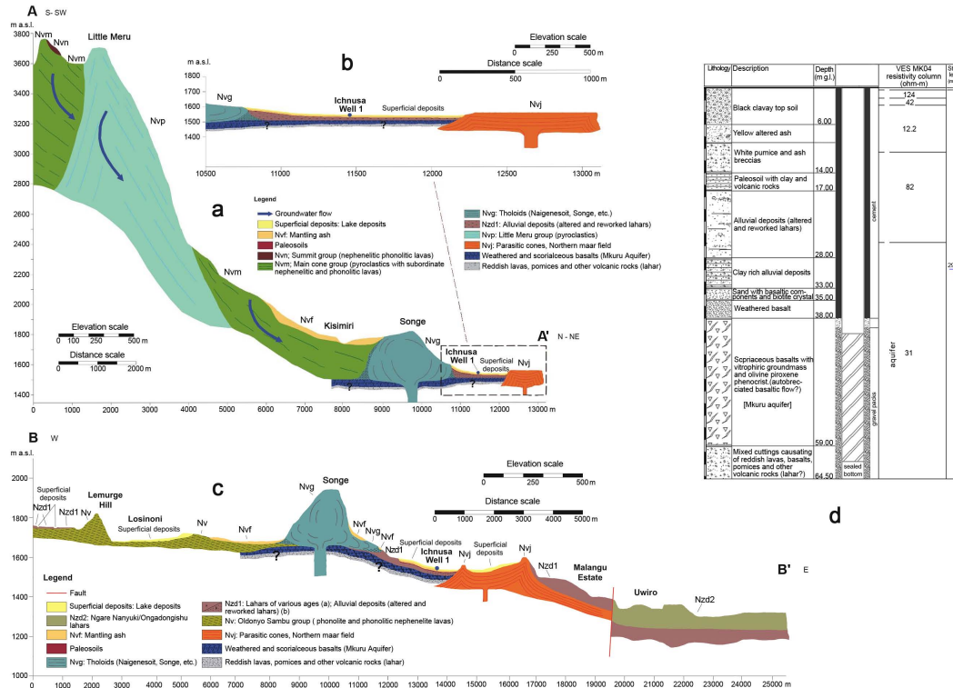
Fig. 6. (a) Geological-Hydrogeological cross section A-A' (vertical exaggeration about x4). (b) Detail of the area surrounding the Ichnusa Well 1. (c) Geological-Hydrogeological cross section B-B' (Vertical exaggeration about x7) (d) – Ichnusa Well 1: lithological log and well construction report. Comparison between the stratigraphy and the resistivity column of the electrical sounding MK04.
