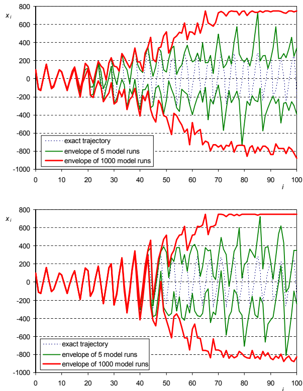
Fig. 6. Stream tube representation of the evolution of soil water x (with initial conditions as in Fig. 4 and 1% uncertainty) in a deterministic setting using envelope curves: (upper) when only x_0 is observed; (lower) when x_0 to x_{30} are observed.
