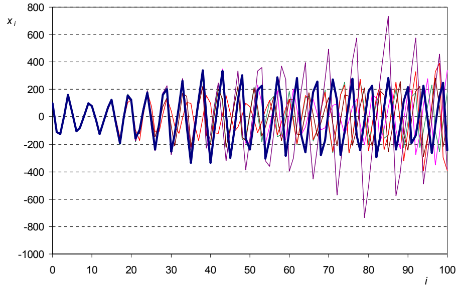
Fig. 5. Evolution of soil water x as in Fig. 4 but with uncertainty in initial conditions: bold blue line corresponds to initial conditions s_0=100 mm, \nu_0=0.30 and the other five lines represent initial conditions slightly ( <1\% ) different.
