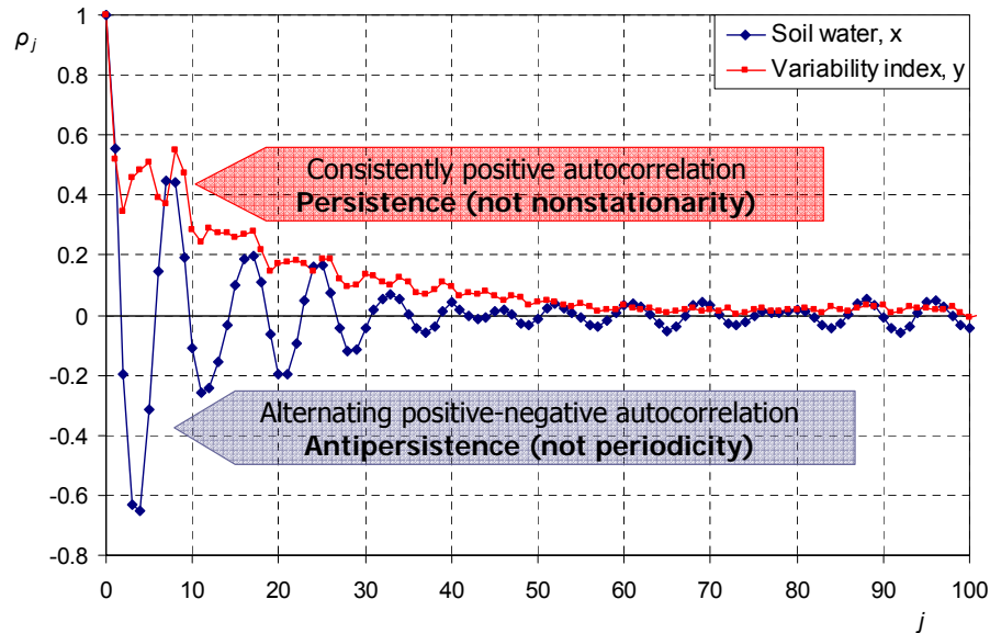
Fig. 14. Empirical autocorrelation functions of 10 000 terms x_j and y_j .
