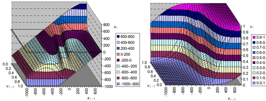
Fig. 3. Graphical depiction of the toy model dynamics.
