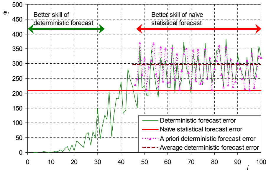
Fig. 10. Comparison of the RMS prediction error of soil water x for the deterministic prediction and the naive statistical prediction.
