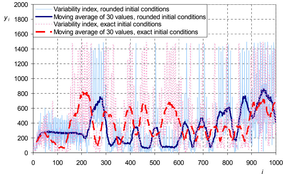
Fig. 16. Plot of 1000 terms of the time series y_i (variability index) at scales 1 and 30 and for two sets of initial conditions deferring less than 1%.
