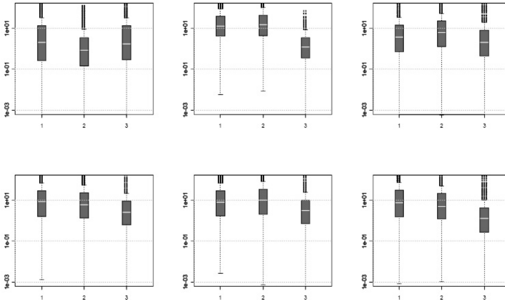
Fig. 12b. Monthly posterior distribution of model specific precision parameter ( \lambda_j ) for three models 1=SDSM, 2=LARS-WG, 3=GEP. Top three plots for July, August, September, bottom three for October, November, December.
