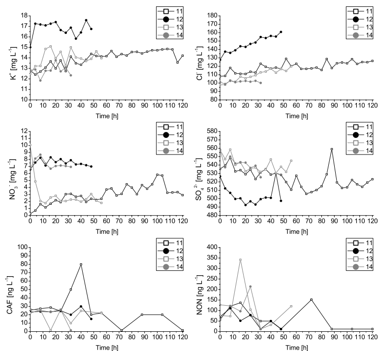
Fig. 2. Concentration-time series for the estimation of M_{CP} with the CSTREAM code. Concentrations are given for inorganic wastewater constituents as well as for caffeine (CAF) and technical-nonylphenol (NON) at the four IPT wells 11, 12, 13 and 14. Concentrations below the LOD were set to half of the LOD.
