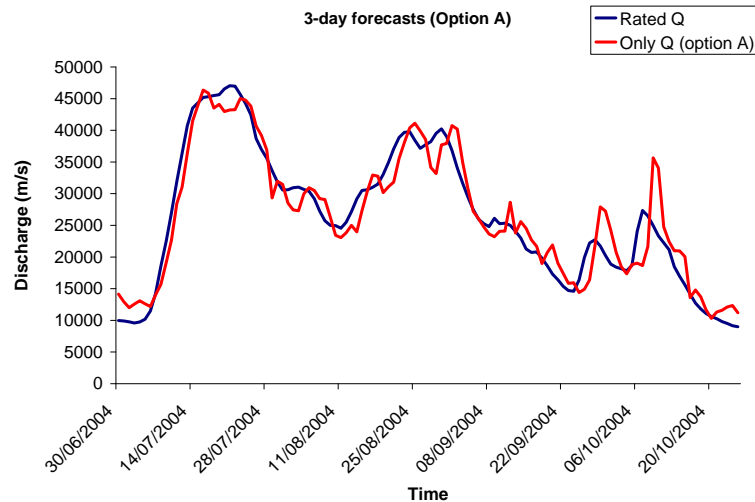
Fig. 4a. Comparison plot of measured discharge with modelled discharge (verification). Option A, only discharge Q.
