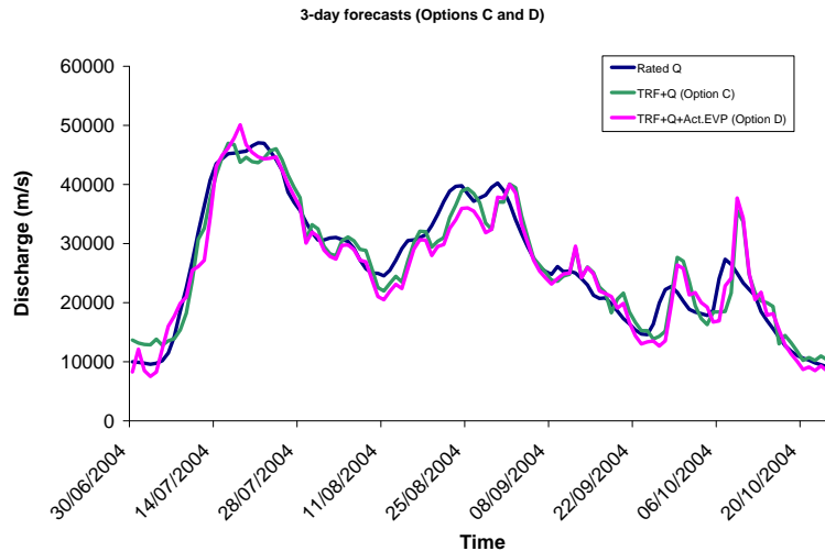
Fig. 4c. Option C (composite rainfall and discharge (TRF+Q)) and D (discharge and actual evapotranspiration, (TRF+Q+Act. Evp).)
