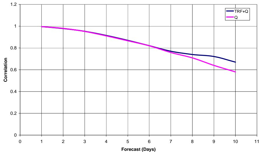
Fig. 6. Comparison of correlation coefficients for Options A (only Q) and Option C (TRF+Q) for extended forecast horizon up to 10 days.
