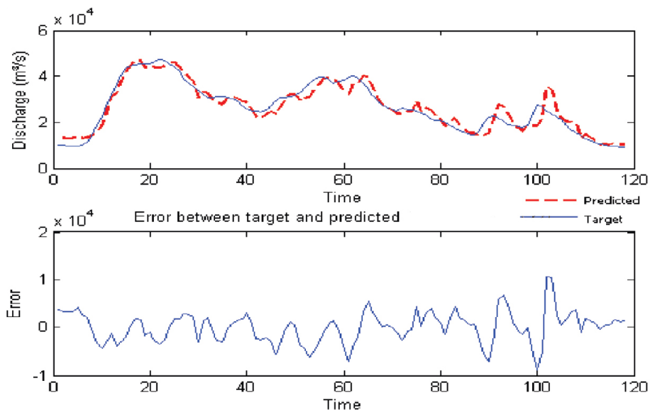
Fig. 5c. Comparison between target and predicted values together with errors (NRMSE) for Option C in verification stage.
