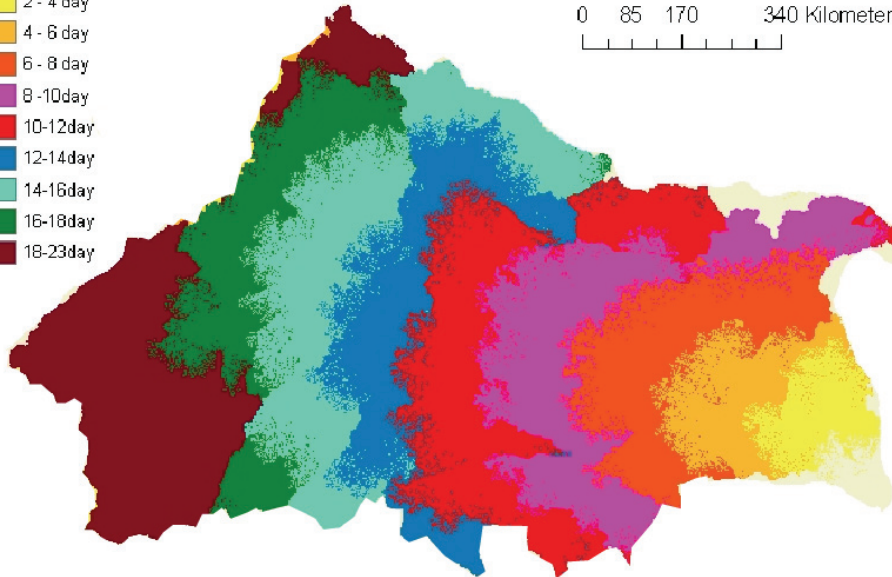
Fig. 3a. Catchment delineation by travel time: conventional average velocity method.
