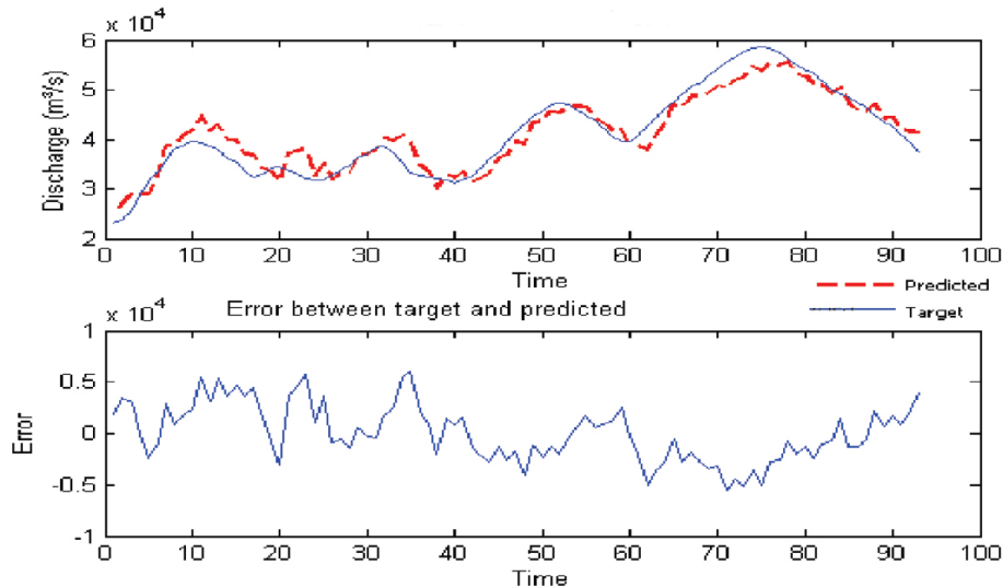
Fig. 5b. Comparison between target and predicted values together with errors (NRMSE) for Option C in cross-validation stage.
