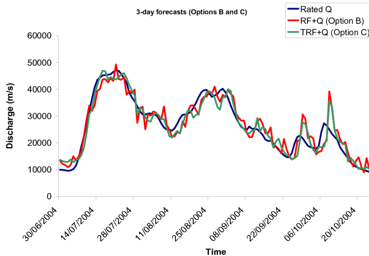
Fig. 4b. Option B (distributed rainfall and discharge (RF+Q)) and C (composite rainfall and discharge (TRF+Q)).
