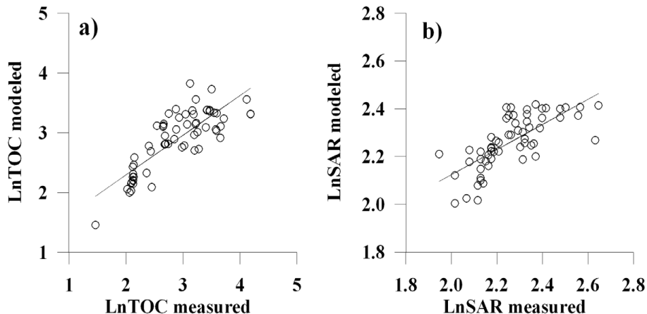
Fig. 5. Plots showing measured and modelled values using partial least square (PLS) models (solid line) for (a) natural logarithm (Ln) of TOC and (b) LnSAR (specific absorption ratio (254/420 nm)). For the TOC PLS model, the factors lake coverage and mire coverage were included, while for the PLS model of SAR, mire coverage and altitude were used. See Methods and Results for more details.
