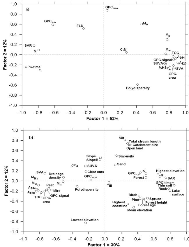
Fig. 4. Common factor analysis plots (based on the structure matrix using Oblimin rotation, \delta=0.6 ) for (a) TOC and NOM character where the factor 1 explains 52% and factor 2, 12% of the variation and (b) physical parameters (from Table 1 plus specific discharge ( q ) and catchment size) together with TOC and NOM character where factor 1 explains 30% and factor 2, 12% of the variation. See Methods for more details and abbreviations.
