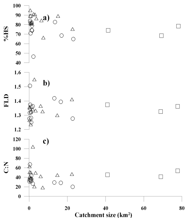
Fig. 3. Aquatic humic substances ( n=28 ): (a) Percentage aquatic humic substances (HS) of DOC (%HS), (b) Fluorescence index (FLD) is the ratio of emission intensity (450 nm: 500 nm) at 370 nm-excitation and (c) C:N variation with catchment size. Data for catchment O, with the branches O1 (○) and O2 (△), and O3 (□). See Methods for more details and abbreviations.
