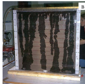
Fig. 8. Fingered flow phenomena in situ and in laboratory experiments. (A) Finger flow in water-repellent sandy soil with permanent grass: 24 h after intensive irrigation the grass layer was removed. Water infiltrates in fingers leaving large sections dry. (B) Evidence of finger flow in laboratory hele-shaw irrigation experiments on dry water repellent sandy soil.
