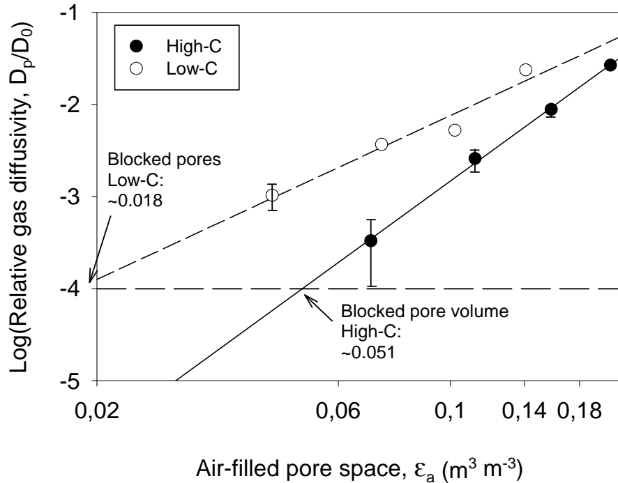
Fig. 3. Gas diffusivity for top layer soil of two arable soils with contrasting contents of management-derived OM (calculated from Schjønning et al., 2002b). Consult text for details.
