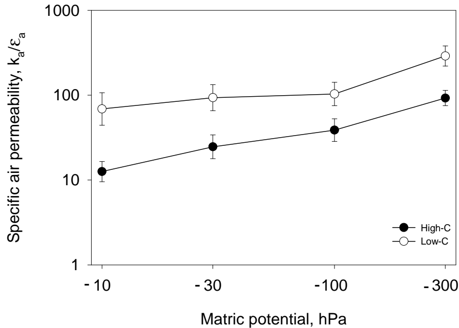
Fig. 5. Specific air permeability ( k_a/\epsilon_a ) at four soil-water matric potentials. Based on data from Schjønning et al. (2002b).
