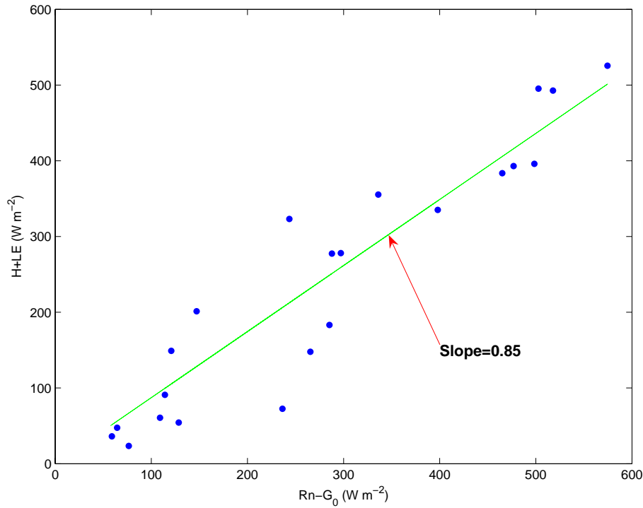
Fig. 5. Comparison between turbulent heat fluxes ( H+LE ) and surface available energy ( Rn-G_0 ) for daytime on 22 June 1998 at the Ando site of the GAME/Tibet experiments.
