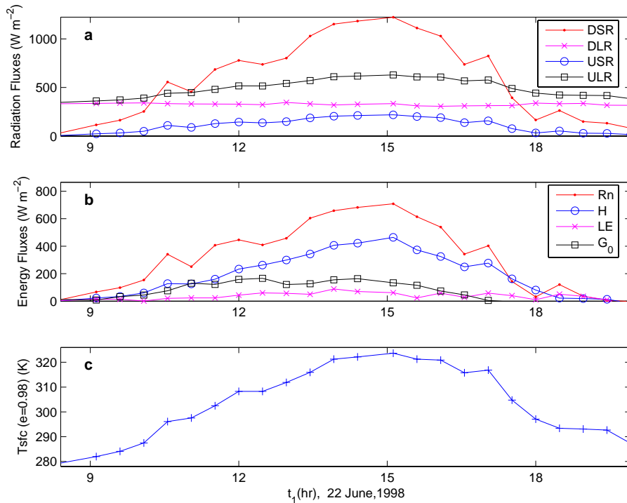
Fig. 4. (a) diurnal variations of surface radiation flux components, i.e., downward shortwave radiation (DSR), downward longwave radiation (DLR), upward shortwave radiation (USR), and upward longwave radiation (ULR) fluxes; (b) same as (a) but for net radiation ( R_n ), sensible heat ( H ), latent heat ( LE ), and soil heat ( G_0 ) fluxes; and (c) surface effective radiative temperature ( T_{sfc} ) which is derived from surface emitted longwave radiation (ULR) with the assurance that the infrared emissivity e=0.98 for daytime on 22 June 1998 at the Ando site of the GAME/Tibet experiments.
