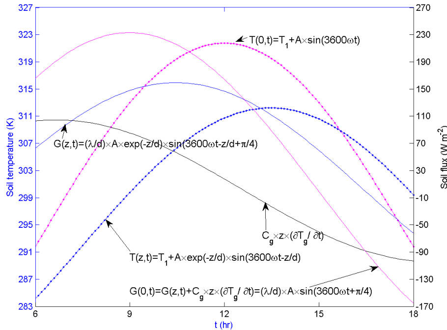
Fig. 1. Theoretical demonstration of temporal variations in soil surface temperature [T(0, t)] , soil temperature [T(z, t)] , soil surface heat flux [G(0, t)] , soil heat flux [G(z, t)] , and soil heat storage C_g z \partial T / \partial t during daytime.
