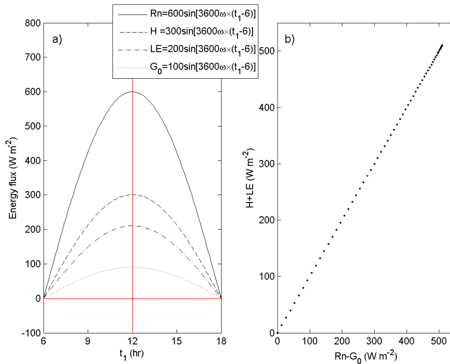
Fig. 2. Theoretical demonstration of (a) temporal variations in surface energy components ( R_n , H , LE , and G_0 ) during daytime, and (b) comparison between turbulent heat fluxes ( H + LE ) and surface available energy ( R_n - G_0 ).
