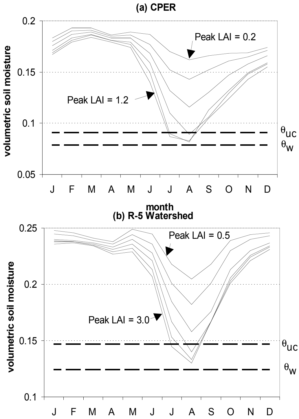
Fig. 8. Sensitivity of modeled root zone soil moisture to the peak in green LAI for: (a) the CPER sandy loam slope in LAI increments of 0.2, and (b) the R-5 watershed in LAI increments of 0.5.
