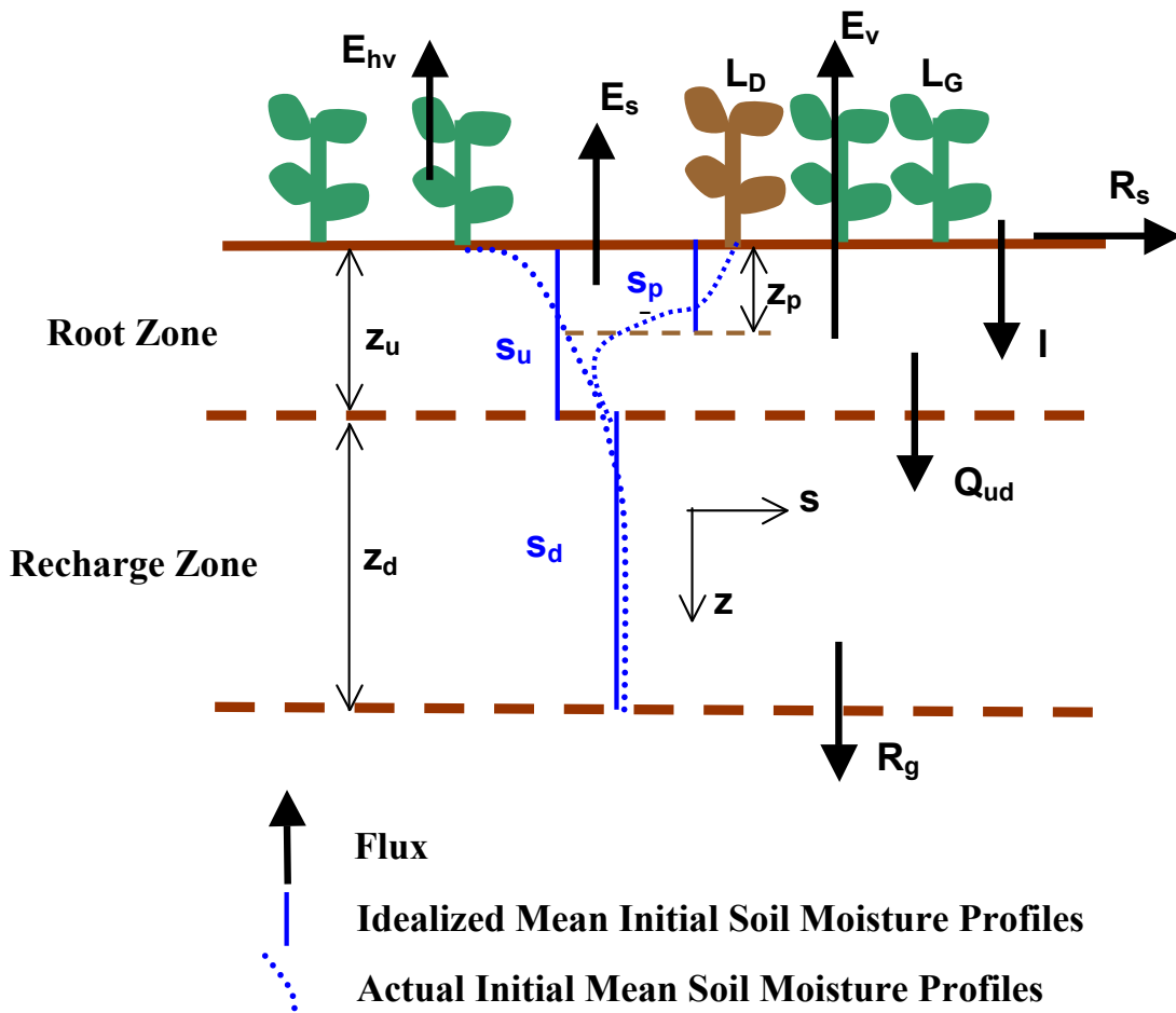
Fig. 2. Schematic of the SDEM.
