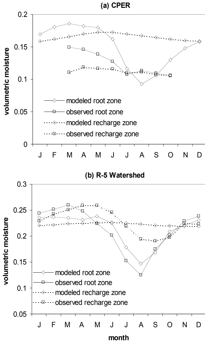
Fig. 9. Comparison of modeled and observed monthly mean soil moisture for: (a) the sandy-loam slope at the CPER, and (b) the R-5 watershed. The observations for Nov.–Feb. at the CPER are not plotted because of infrequent measurements (see Fig. 7a). The fact that observed spring recharge at the CPER is less than modeled is likely due to the first measurement being taken at a depth of 30 cm. For a discussion of other discrepancies between modeled and observed soil moisture see Section 7.
