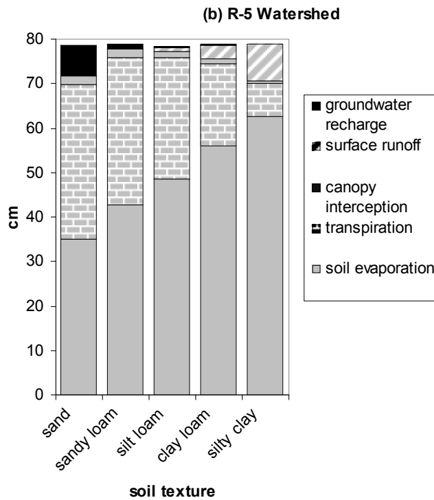
Fig. 12. Sensitivity of the components of the annual water balance to variations in soil texture for: (a) the CPER, and (b) the R-5 watershed.
