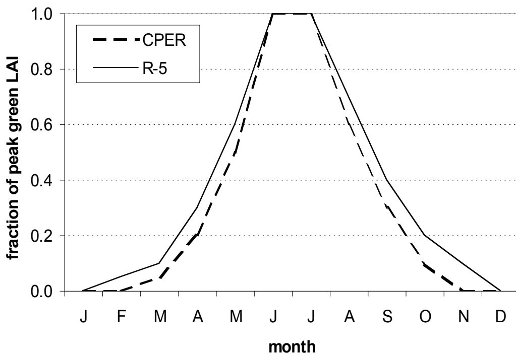
Fig. 7. Phenology of green LAI. The wider curve for the R-5 watershed is reflective of a longer growing season.
