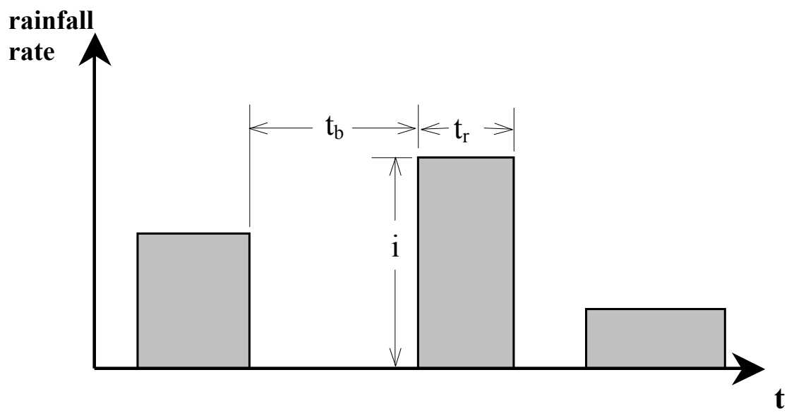
Fig. 1. The rectangular pulse model of precipitation.
