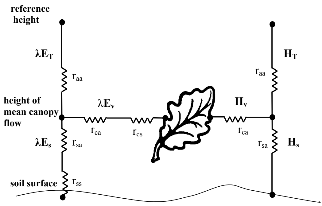
Fig. 5. Schematic of the Shuttleworth-Wallace (1985) two-component canopy model.
