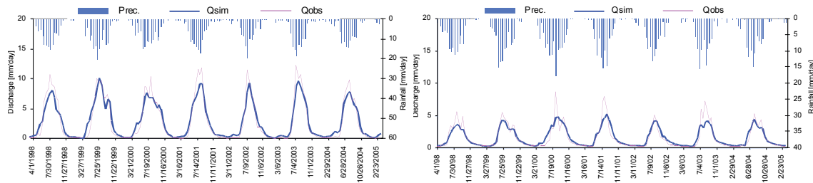
Fig. 3. Simulated and observed stream flow hydrographs for the 15-days time step models (CR III).
