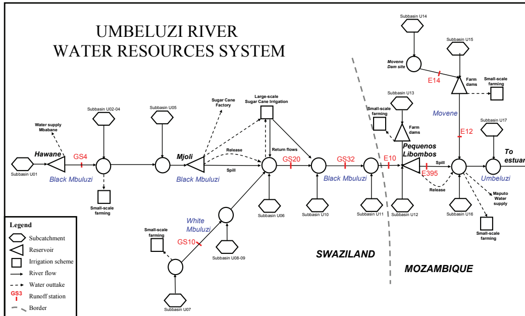
Fig. 2. Simplified Umbeluzi River basin system model schematic.
