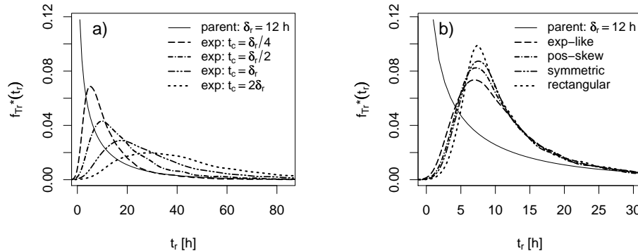
Fig. 7. Effect of the response time t_c (a) and the shape of the UH (b) on the flood-producing storm durations. The black continuous line is the parent distribution, given in Eq. (2) with mean storm duration \delta_r=12 h and coefficient of variation CV_r \approx 1.46 ( \beta_r=0.7 ), while the other lines are the distributions of the durations of flood-producing storms. In panel (a) the UH is a linear reservoir (see Eq. 8) with response time t_c=3, 6, 12, 24 h; in panel (b) the UHs have different shapes given by beta distributions with shape parameters p_\beta and q_\beta : exponential like ( p_\beta=1, q_\beta=4 , width of 17 h); positively skewed distribution ( p_\beta=2, q_\beta=4 , width of 12 h); symmetric distribution ( p_\beta=2, q_\beta=2 , width of 9 h); rectangular ( p_\beta=1, q_\beta=1 , width of 7 h).
