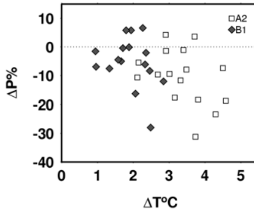
Fig. 4. Change in precipitation versus change in temperature for the 16 GCM projections under the two emissions scenarios for the Rio Lempa basin. Changes are between 1961–1990 and 2070–2099.
