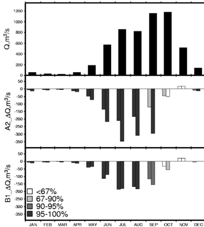
Fig. 6. Climatological (1961–1990) inflow to at 15 Setiembre, and projected changes. Shading and symbols are identical to Fig. 5.
