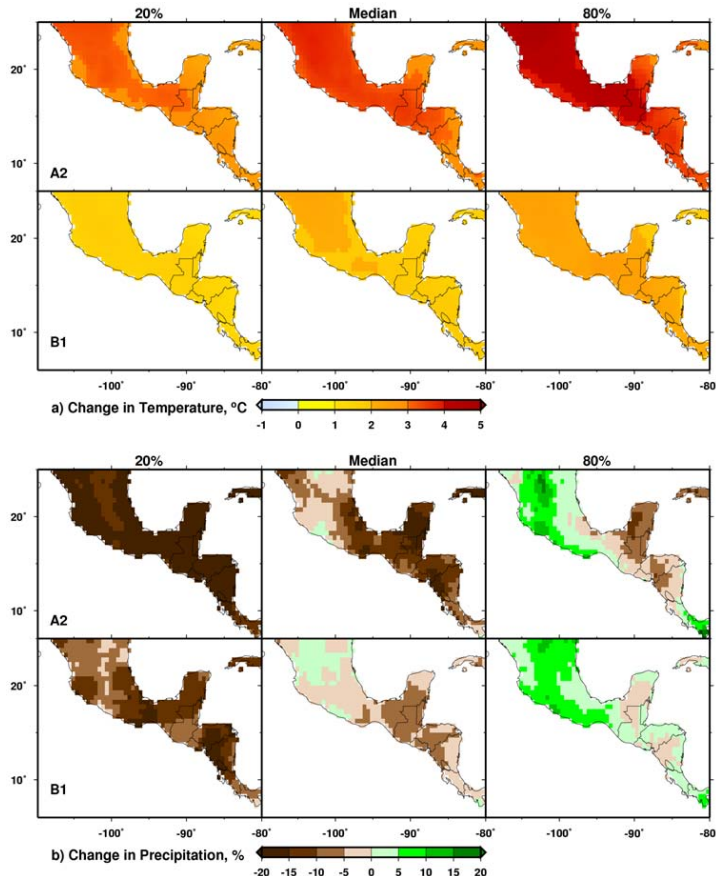
Fig. 3. (a) Projected temperature change and (b) precipitation change for Central America from 1961–1990 and 2070–2099 under higher (A2) emissions (upper row) and lower (B1) emissions (lower row). For the ensemble of 16 GCMs, 20, 50, and 80 percent non-exceedance values are shown in the three columns.
