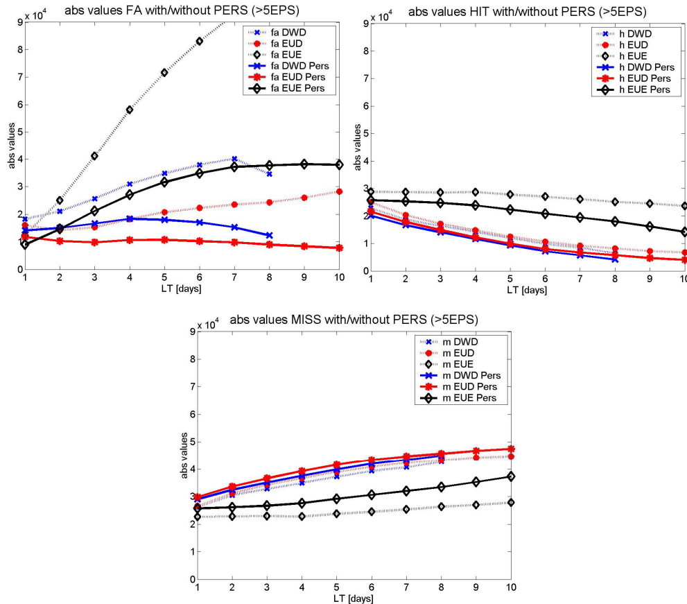
Fig. 2. Absolute numbers of “false alerts f” (top left), “hits h” (top right) and “misses m” (bottom) for deterministic forecasts (DWD and EUD) and at least 5 EPS > HAL (EUE) over leadtime, with (full line) and without (dotted line) persistence.
