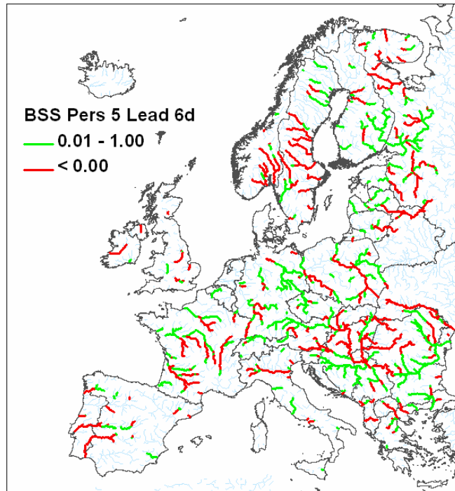
Fig. 8. Areal distribution of BSS median values for 6 days of leadtime and persistence (>5 EPS).
