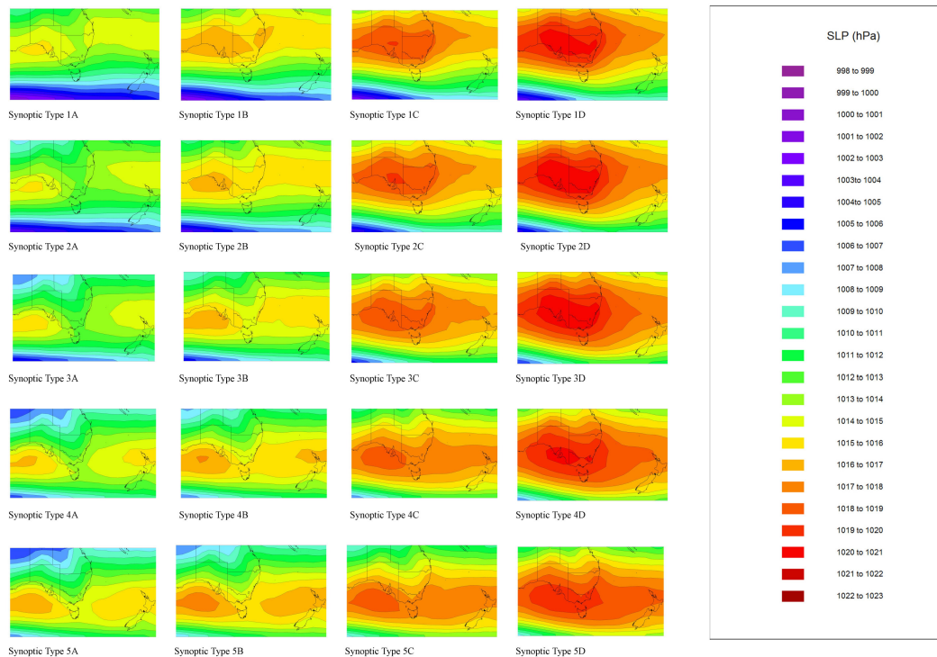
Fig. 3. 20 key regional synoptic patterns characterised using SOM.
