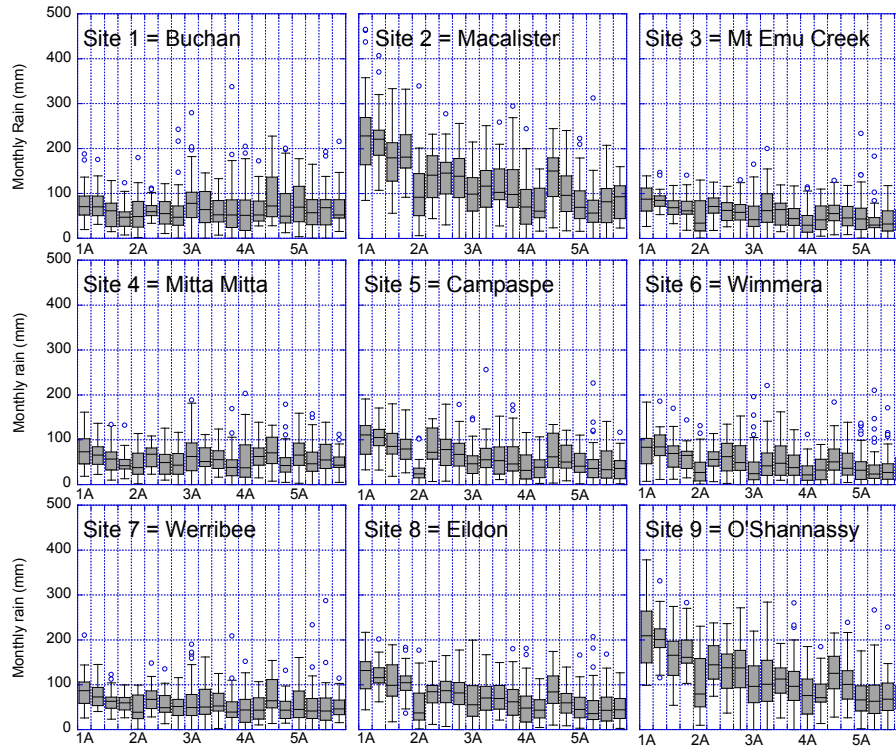
Fig. 5. Box plots of monthly rainfall associated with each of the 20 synoptic types.
