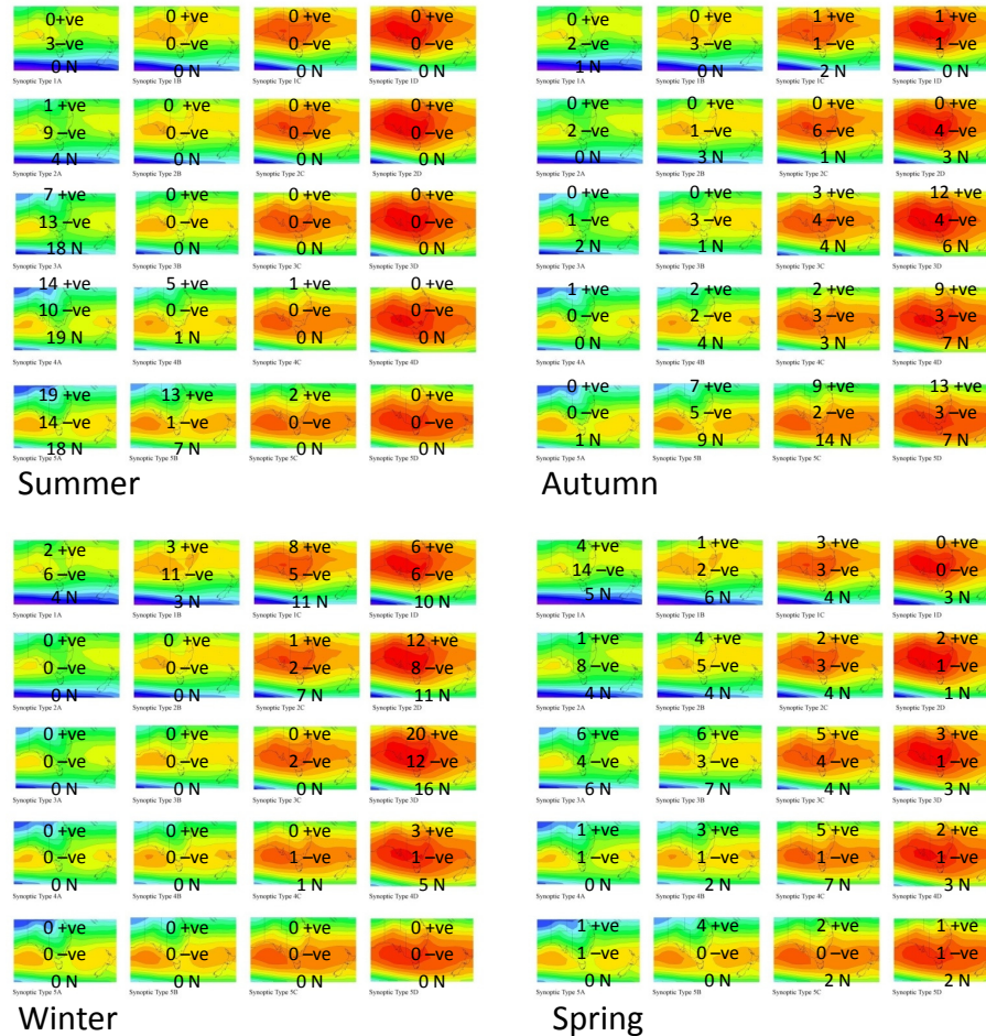
Fig. 8. Number of times each synoptic type has occurred since 1948 on a seasonal basis, stratified into SAM positive (+ve), SAM negative (-ve) and SAM neutral (N) phases.
