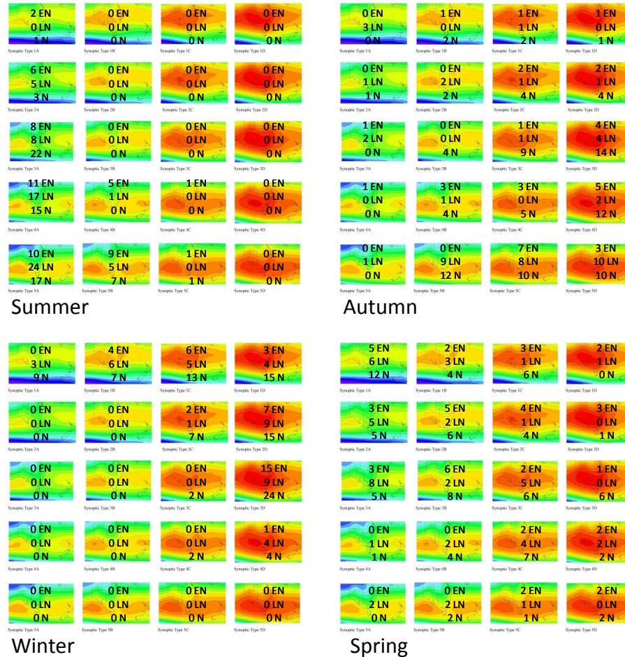
Fig. 6. Number of times each synoptic type has occurred since 1948 on a seasonal basis, stratified into El Niño (EN), La Niña (LN) and Neutral (N) phases.
