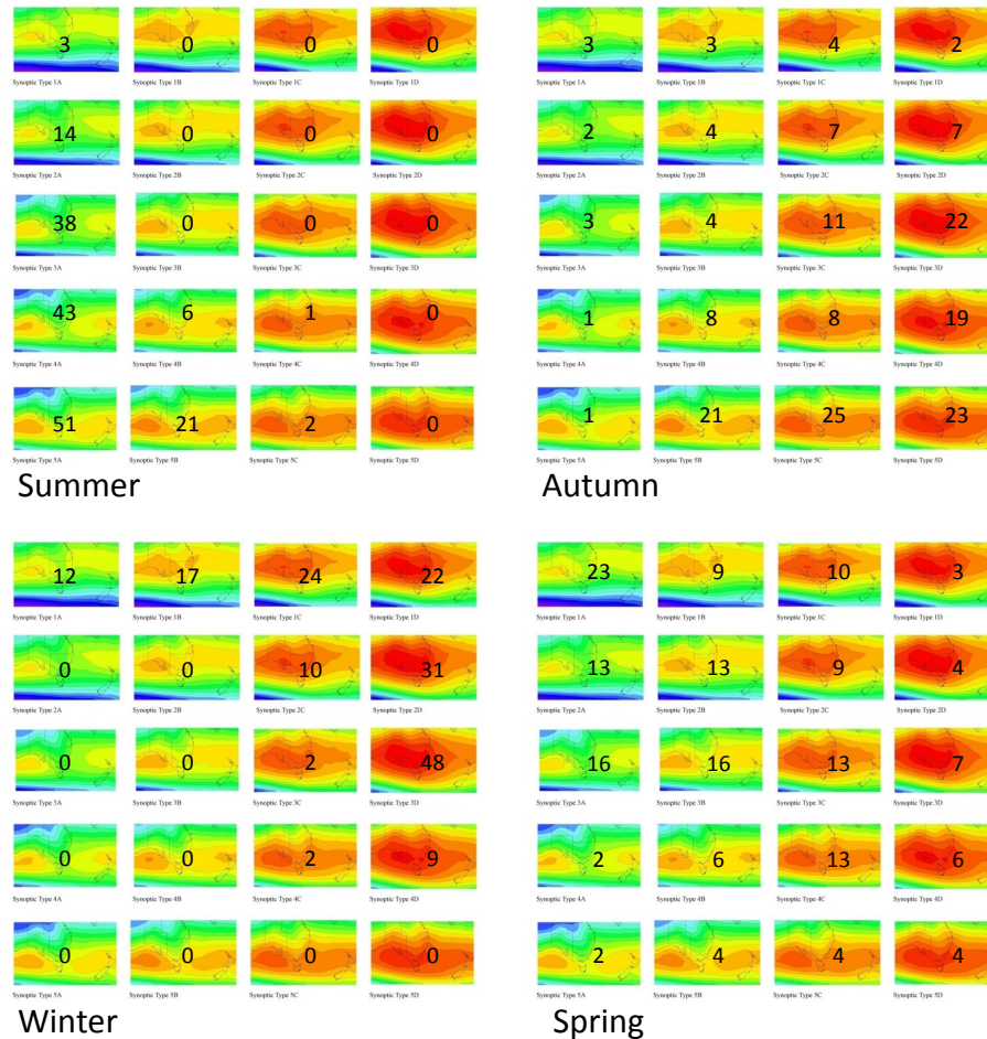
Fig. 4. Number of times each synoptic type has occurred since 1948 on a seasonal basis.
