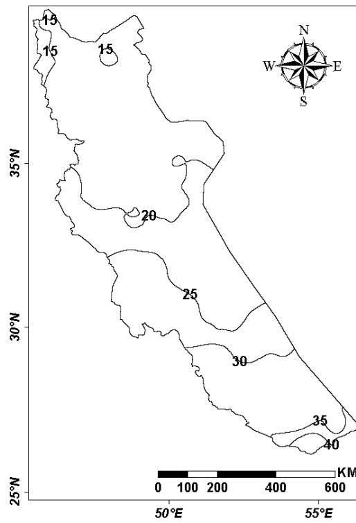
Fig. 5. Spatial distribution of PCI in western Iran.
