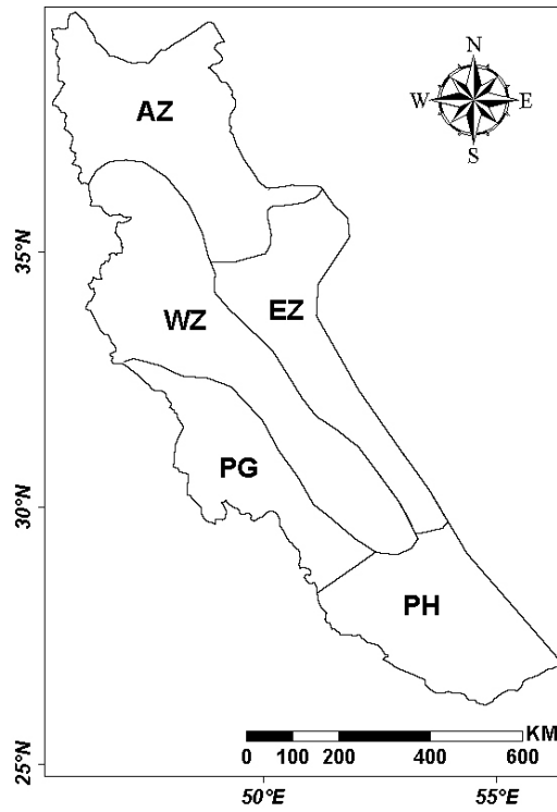
Fig. 8. Precipitation-based regionalization in western Iran.
