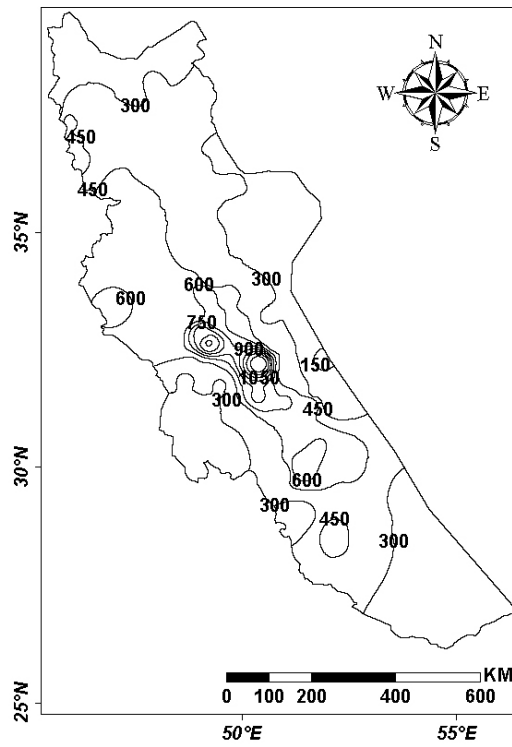
Fig. 2. Spatial distribution of the mean annual precipitation in western Iran. Unit is mm.
