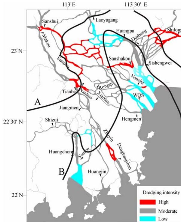
Fig. 5. River channels dominated by different intensity of the in-channel sand dredging. The solid lines marked with A and B show the demarcation of flood and flood-tidal areas (line A) and the demarcation of flood-tidal and tidal areas (line B) (after Huang et al., 1999). WQS: the Wanquanshaxi station.
