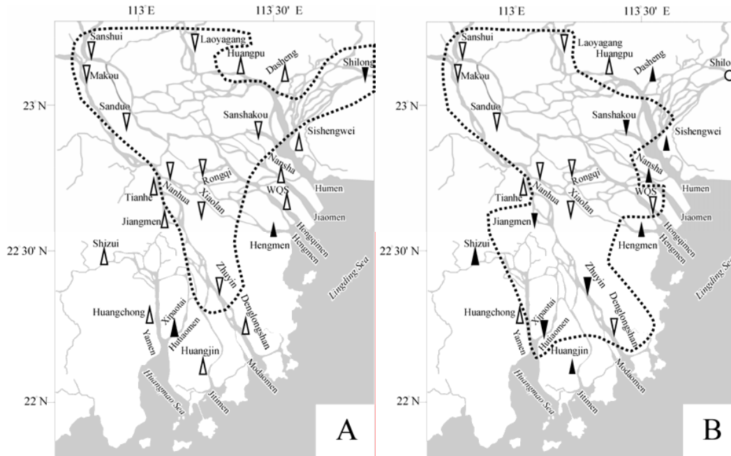
Fig. 3. Variations of the extreme high (A) /extreme low (B) water level exceeding mean + std threshold in summer. The triangles denote increasing/decreasing relative frequency of high/low water level (no trend); The solid triangles denote significant increasing/decreasing trend of the relative frequency of the high/low water level. The circles denote zero frequency. Stations dominated by decreasing water level are circled by dashed lines. WQS is the abbreviation of the Wangquanshaxi station.
