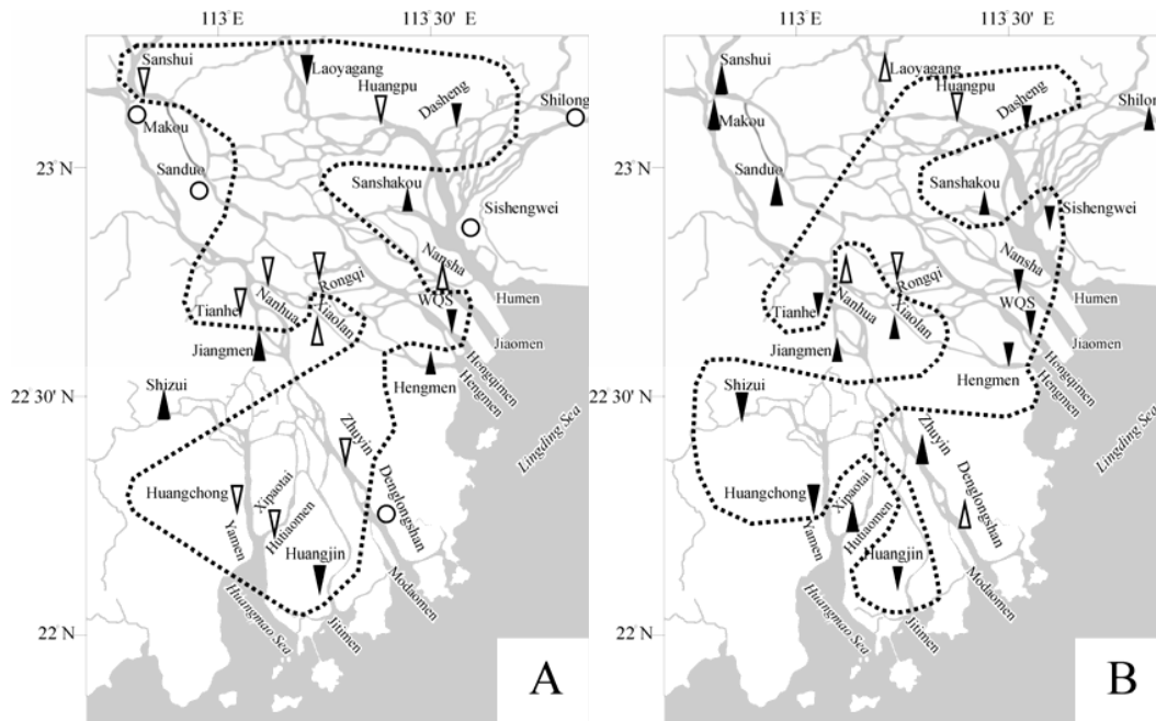
Fig. 4. Variations of the extreme high (A)/extreme low (B) water level falling below mean – std threshold in winter. The triangles denote increasing/decreasing relative frequency of high/low water level (no trend); The solid triangles denote significant increasing/decreasing trend of the relative frequency of the high/low water level. The circles denote zero frequency. Stations dominated by decreasing water level are circled by dashed lines. WQS is the abbreviation of the Wangquanshaxi station.
