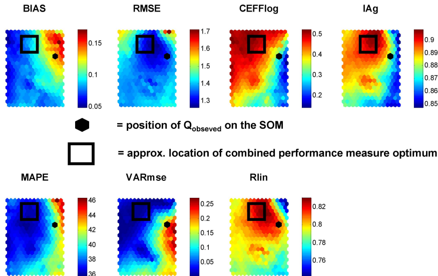
Fig. 4. The location of the best-matching unit (indicated by the black dot) for an input vector that represents the measured discharge time series. The rectangle outlines the region on the map where approximately a combined optimum of the seven performance measures has to be expected.
