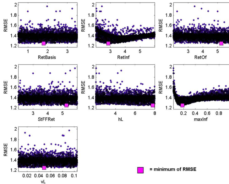
Fig. 3. Scatterplots of RMSE values for each of the examined NASIM parameters.
