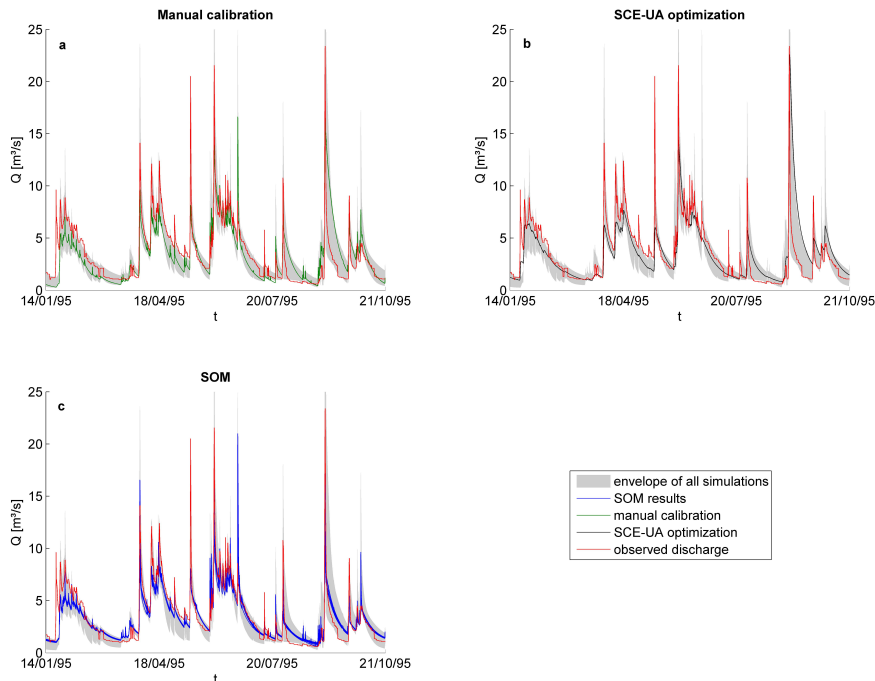
Fig. 5. The model realizations as resulting from (a) manual calibration, (b) optimization with the SCE-UA algorithm and (c) the BMU of the SOM for the measured discharge time series. The time-series are compared to the measured discharge and the envelope of the Monte-Carlo simulation, i.e. the area which is spanned by all model time series for the bounds given in Table 1.
