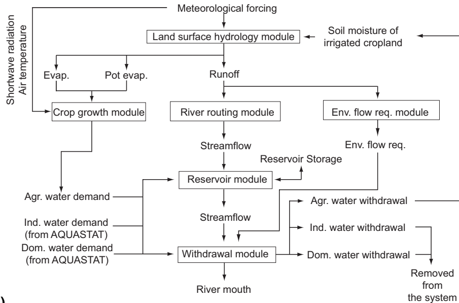
Fig. 1. Schematic diagram of water flow among modules.
