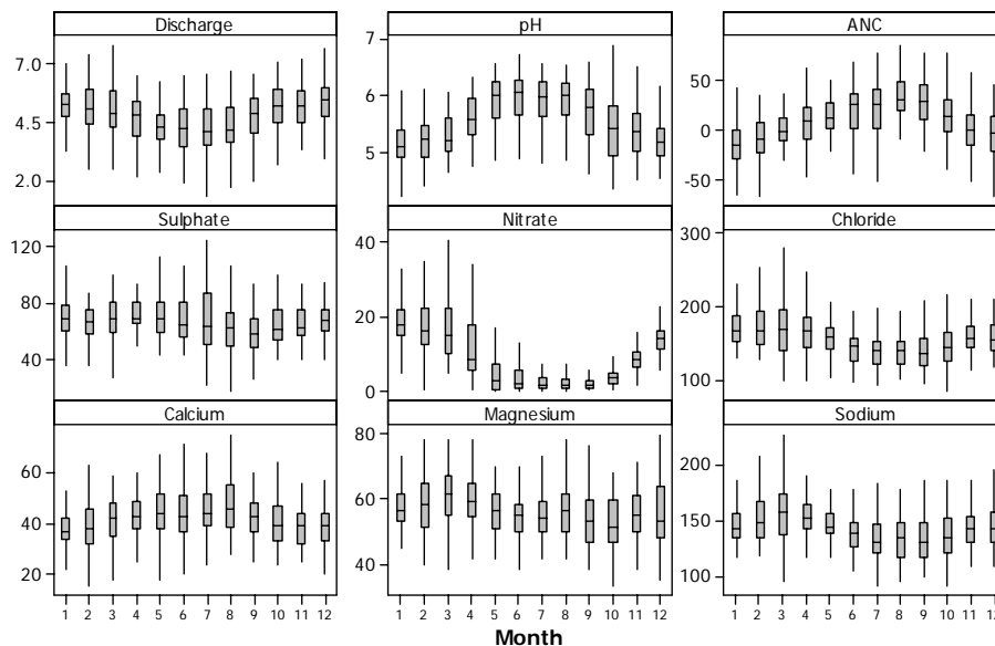
Fig. 3. Monthly box and whisker plots for stream discharge (natural log of discharge in \text{ls}^{-1} ), pH (pH units), Acid Neutralising Capacity and major ions (all \text{eq l}^{-1} ). For each month, central line represents median, boxes 25th and 75th percentiles, and whiskers 10th and 90th percentiles. Months numbered from January to December.
