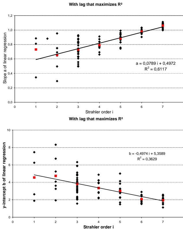
Fig. 5. Relationship to Strahler order of the slope (top) and y-intercept (bottom) of the linear regression between WT and lagged AT, using the lag that maximizes the determination coefficient R 2 . The black lines are the regression lines between the Strahler orders and the means of the slope and y-intercept for each Strahler order, represented by red squares. They are characterized by the linear regression equations and determination coefficients given in the plots.
