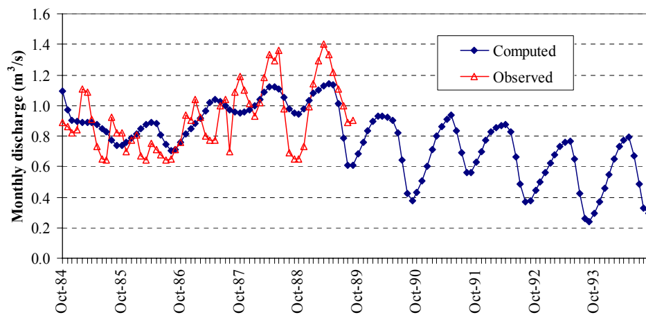
Fig. 13. Computed and observed discharge series at Polygyra springs.
