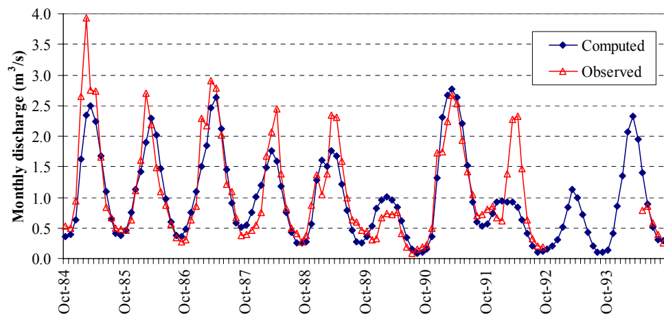
Fig. 8. Computed and observed discharge series at Lilaia-Kefalovrysso springs.
