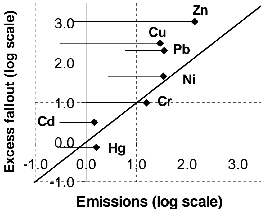
Fig. 5. Comparison of measured atmospheric fallout, corrected from soil dust resuspension, to declared and aggregated atmospheric emissions over the whole Seine River basin ( \text{t y}^{-1} ) (bars represent emission uncertainties) (data from Thévenot et al., 2007).
