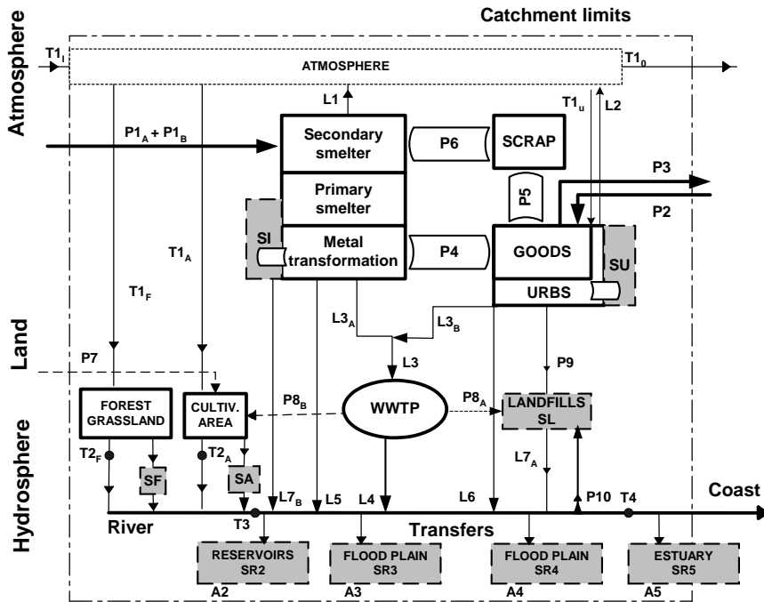
Fig. 2. Schematic sources, transfers, sinks of metals in a river catchment combined with metal uses, recycling and leaks in the anthroposphere. P1 to P10: circulation of metal products and goods. L1 to L7: leaks from the anthroposphere to the environment. T1 to T4: transfers. SA to SU: storage. A: sediment archives of past river contamination. Grey area: metal storage sites. (•): River stations. (WWTP): waste water treatment plants (see also Tables 1, 2, 3).
