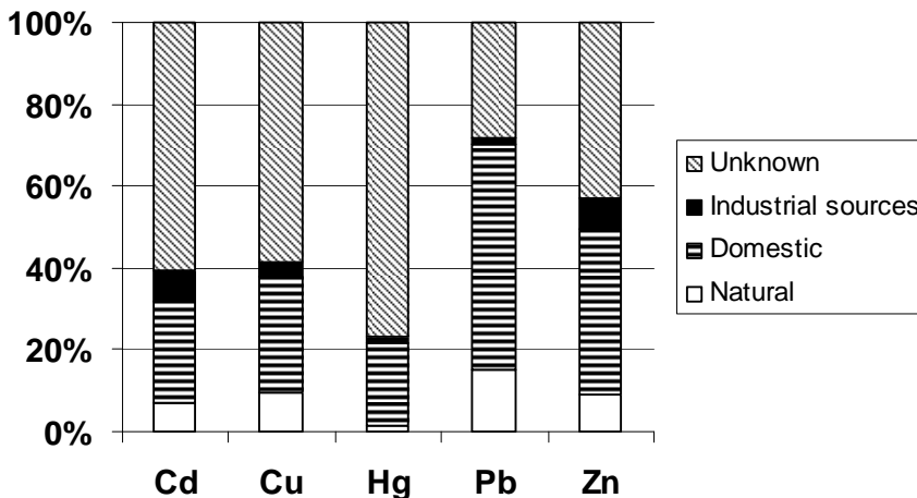
Fig. 6. Percentage of metal sources Cd, Cu, Hg, Pb, Zn, in total export at the river mouth station Poses: (i) release from erosion (“natural”), (ii) calculated domestic release (“domestic”) and (iii) directly measured or declared direct release of industrial waste water into rivers, (iv) unknown sources.
