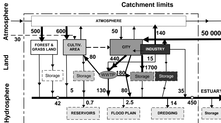
Fig. 4. Zinc budget in the Seine basin : mean fluxes and flows during the 1994–2003 period ( \text{ty}^{-1} ) (data from Thévenot et al., 2007).
