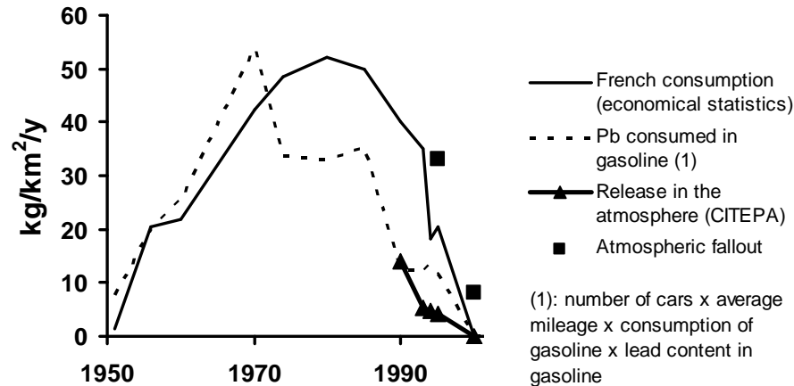
Fig. 3. Long term trend of leaded gasoline in atmosphere (flows/fluxes in kg/km 2 /y).
