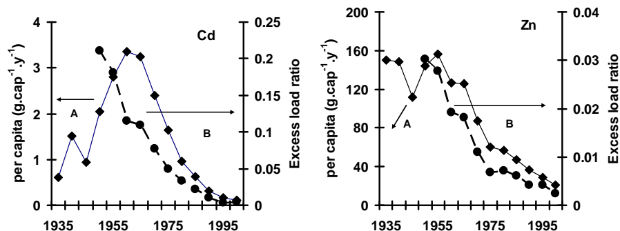
Fig. 7. Integrated F2A indicators for Cd (left) and Zn (right). A: Annual average river excess metal load prorated to the Seine basin population ( \text{g cap}^{-1} \text{y}^{-1} ). B: Annual export by the river/total metal demand in the catchment (leakage ratio) (data from Meybeck et al., 2007).
