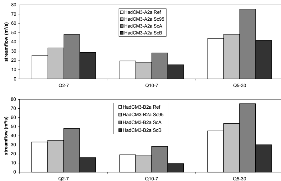
Fig. 9. Effect of CC (Sc95 vs. ref) and land use evolution scenarios (ScA and ScB vs. Sc95) on low flow statistical sequences ( m^3/s ) obtained with downscaling method and the two GCM-GES-M used (HadCM3-A2a and HadCM3-B2a).
