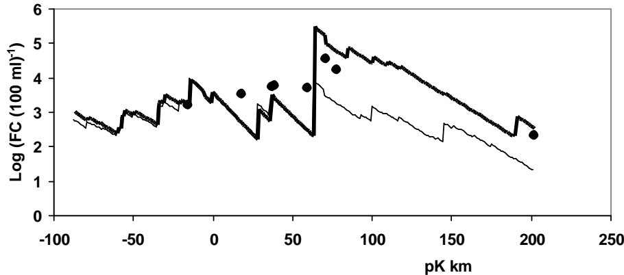
Fig. 6. Longitudinal variations in summer conditions of FC abundance calculated by the FC-SENEQUE model for the year 2003 (bold line) and for the year 2012 (prospective scenario)(fine line) in the Seine river between the confluence of the Seine with the Yonne river (pK –88) and the entrance of the estuary (pK 202). Average field data (black dots) for the summer 2003 period are also plotted (SIAAP and SNS, personal communication). pK is a kilometric unit that is set at zero at “Pont Marie” in Paris downtown and increases from upstream to downstream (negative values are thus for stations upstream Paris).
