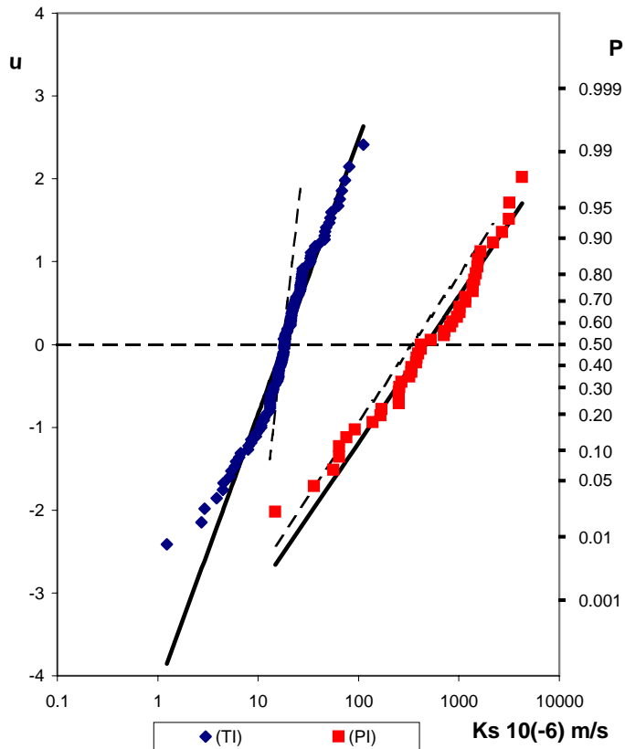
Fig. 3. Fractil diagram of the k_s values by the log-normal distribution, for two wide data sets relative to the (TI) (126 data) and (PI) (45 data) methods and comparison between the correspondent distributions relative to reduced sets of 23 data.
