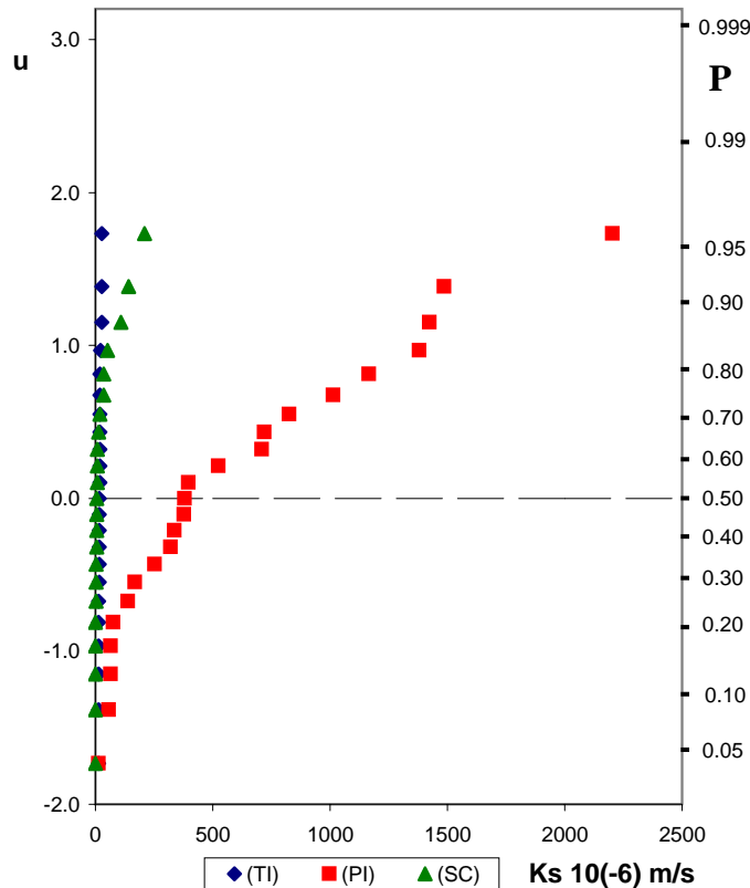
Fig. 1. Fractil diagram of the k_s values by the normal distribution, for the (TI), (PI) and (SC) measurement methods.
