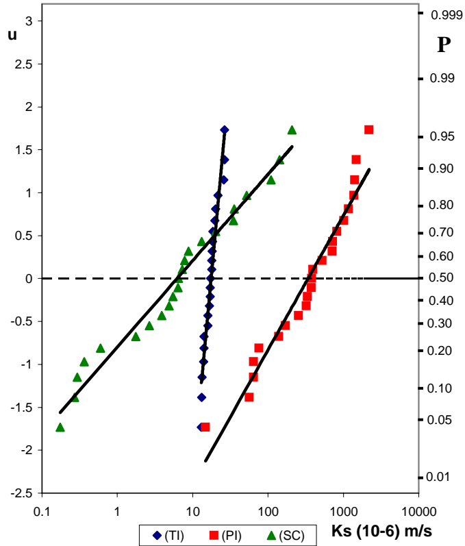
Fig. 2. Fractil diagram of the k_s values by the log-normal distribution, for the (TI), (PI) and (SC) measurement methods.
