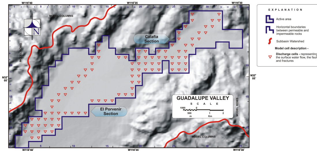
Fig. 6. Cell location representing discharge cell by the surface water flow, as well as the faults and fractures used as discharge cells assigned in the groundwater flow model of the Guadalupe Valley.
