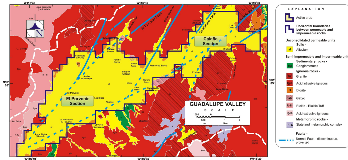
Fig. 3. Regional geology of the Guadalupe Valley Region (INEGI, 1976).
