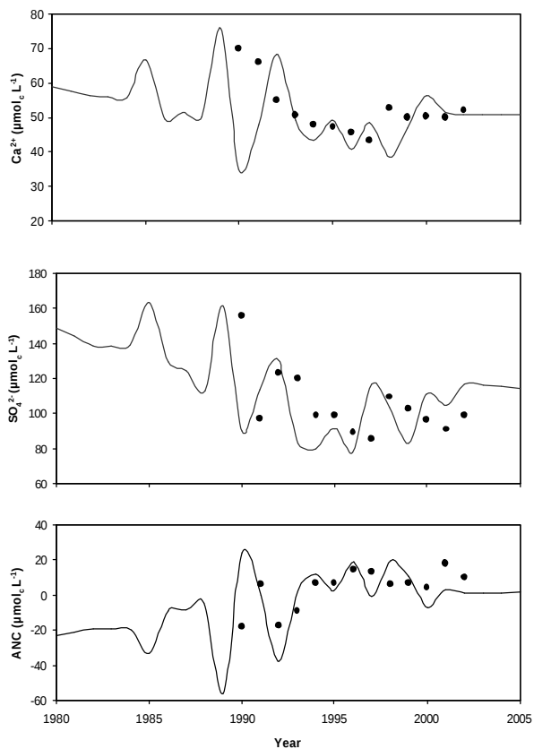
Fig. 4. MAGIC simulation (solid line) calibrated to long-term time-series (1990–2002) of observed data (solid circles) for \text{Ca}^{2+} , \text{SO}_4^{2-} and \text{ANC} ( \mu\text{mol}_c \text{L}^{-1} ) at Little Wiles Lake.
