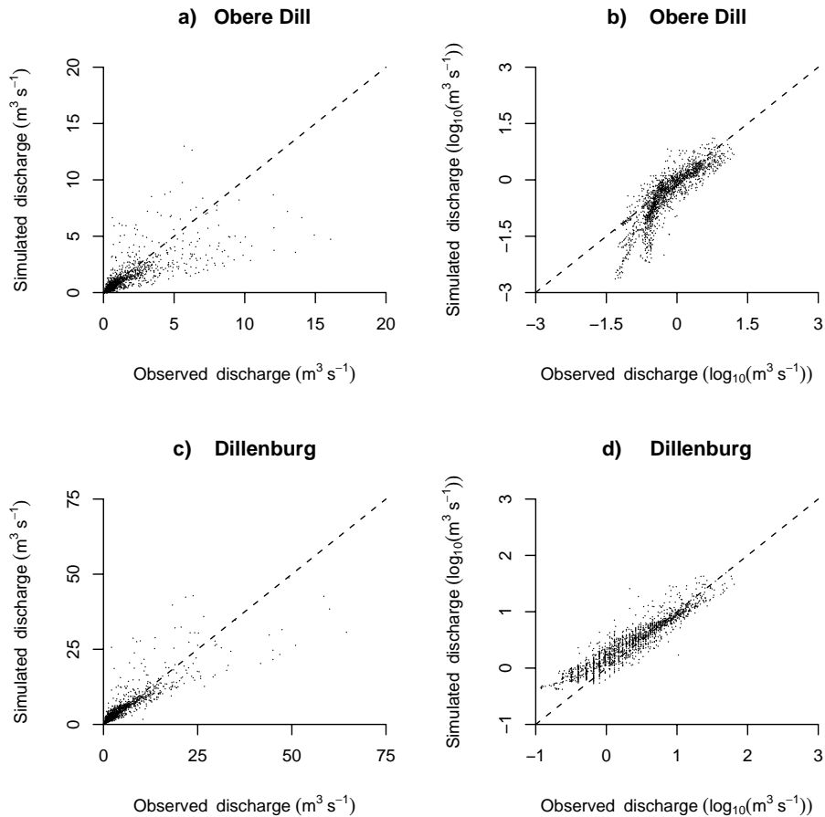
Fig. 4. Scatterplots of simulated and observed discharge at gauges Obere Dill and Dillenburg. Daily discharge (left) and log-transformed daily discharge (right) are depicted for the period 1 July 2000 to 31 December 2004. The dashed line indicates the one-to-one line.
