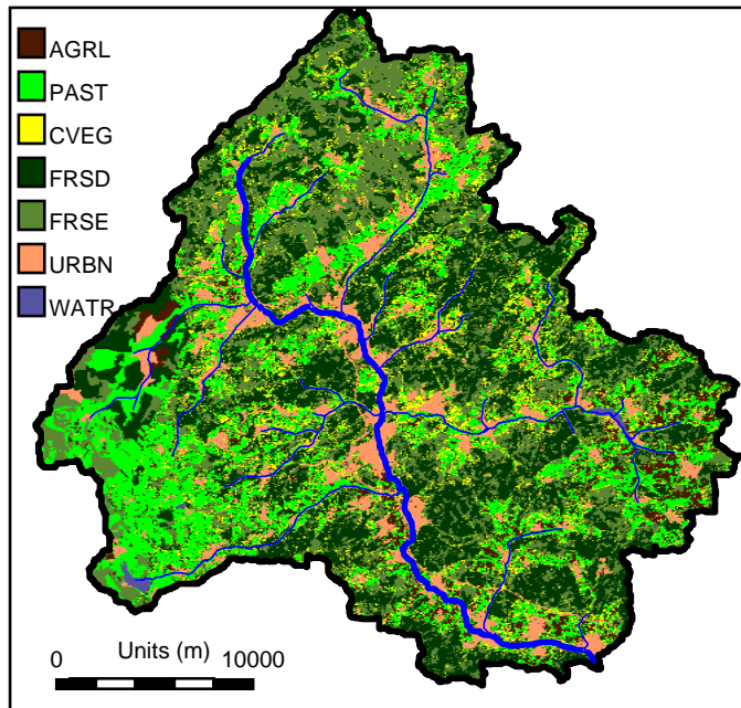
Fig. 1. Map of actual land-use in the Dill catchment based on LANDSAT TM5 data (Nöhles, 2000). AGRL means arable land, PAST is pasture, CVEG is changing vegetation, FRSD is deciduous forest, FRSE is evergreen forest, URBN means urban area, and WATR denotes surface water.
