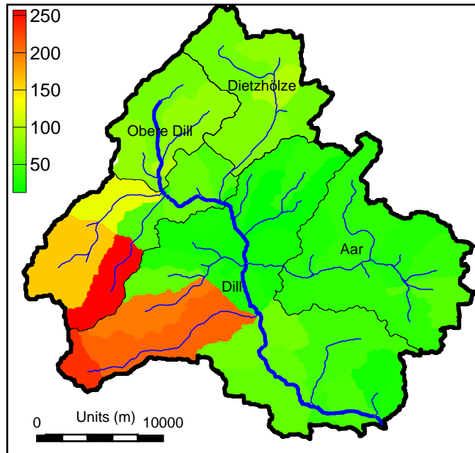
Fig. 5. Map of simulated annual average groundwater contribution to the reach of each sub-basin (2000–2004).
