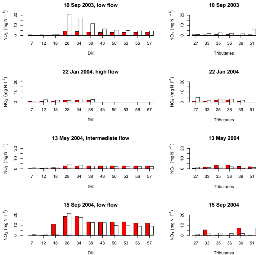
Fig. 8. Comparison of observed (white) and simulated (red) nitrate concentrations at various sampling locations along the river channel Dill (left) and at various tributaries (right) on four different dates. The sampling sites are given in Fig. 3.
