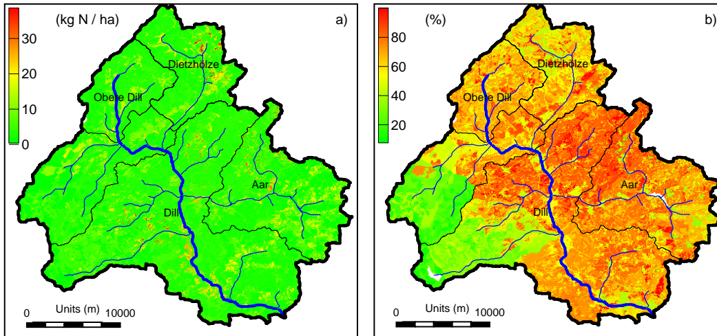
Fig. 9. Simulated average annual nitrate leaching through lateral flow ( \text{kg N ha}^{-1} ) for 2000 to 2004 (left). Ratio between nitrate leaching through lateral flow and total nitrate leaching (%) for the same period (right).
