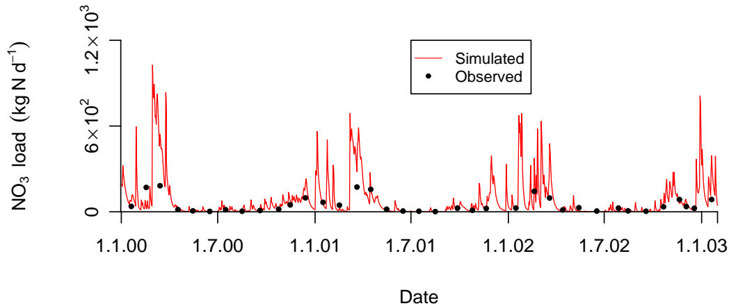
Fig. 7. Simulated and observed daily nitrate load at gauge Obere Dill (1 January 2000–28 February 2003).
