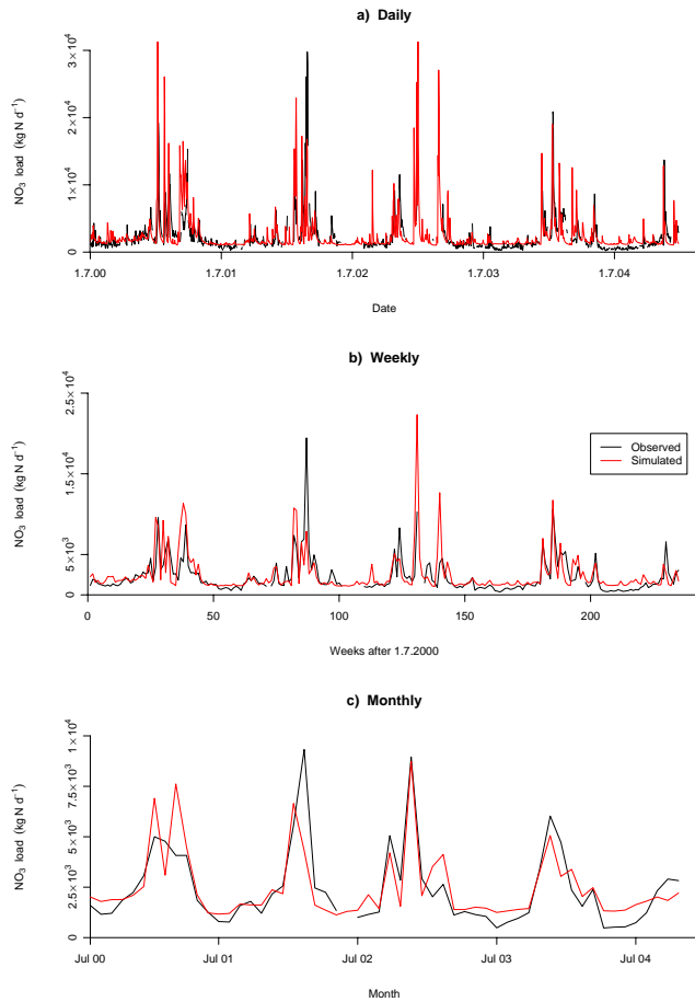
Fig. 6. Simulated and observed nitrate load at gauge Aßlar (1 July 2000–31 December 2004).
