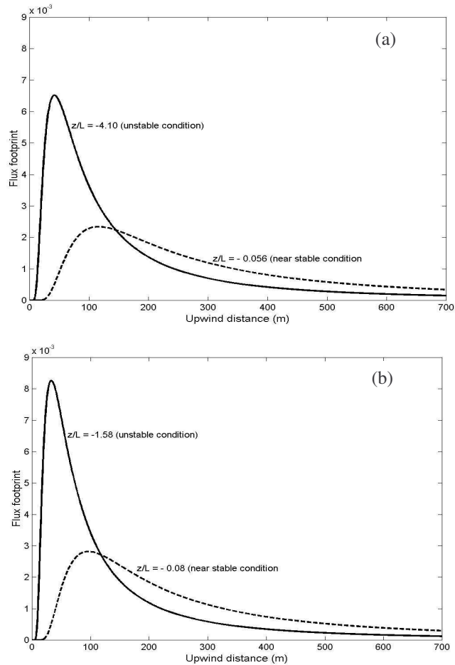
Fig. 5. Footprint representation for two selected days in the dry season and rainy season: (a): DOY 31 (dry season) at 13:00 (unstable condition) and at 08:00 (near stable condition) (b): DOY 179 (rainy season) at 12:00 (unstable condition) and 08:00 (near stable condition).
