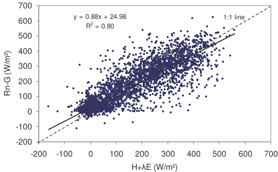
Fig. 2. Energy balance closure for the whole dataset (from January to November 2004).
