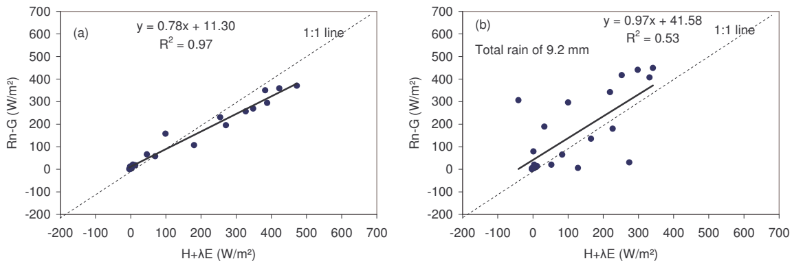
Fig. 4. Energy balance closure for two selected days during the rainy season: (a) DOY 170 without rain and (b) DOY 168 with a total rainy of 9.2 mm.
