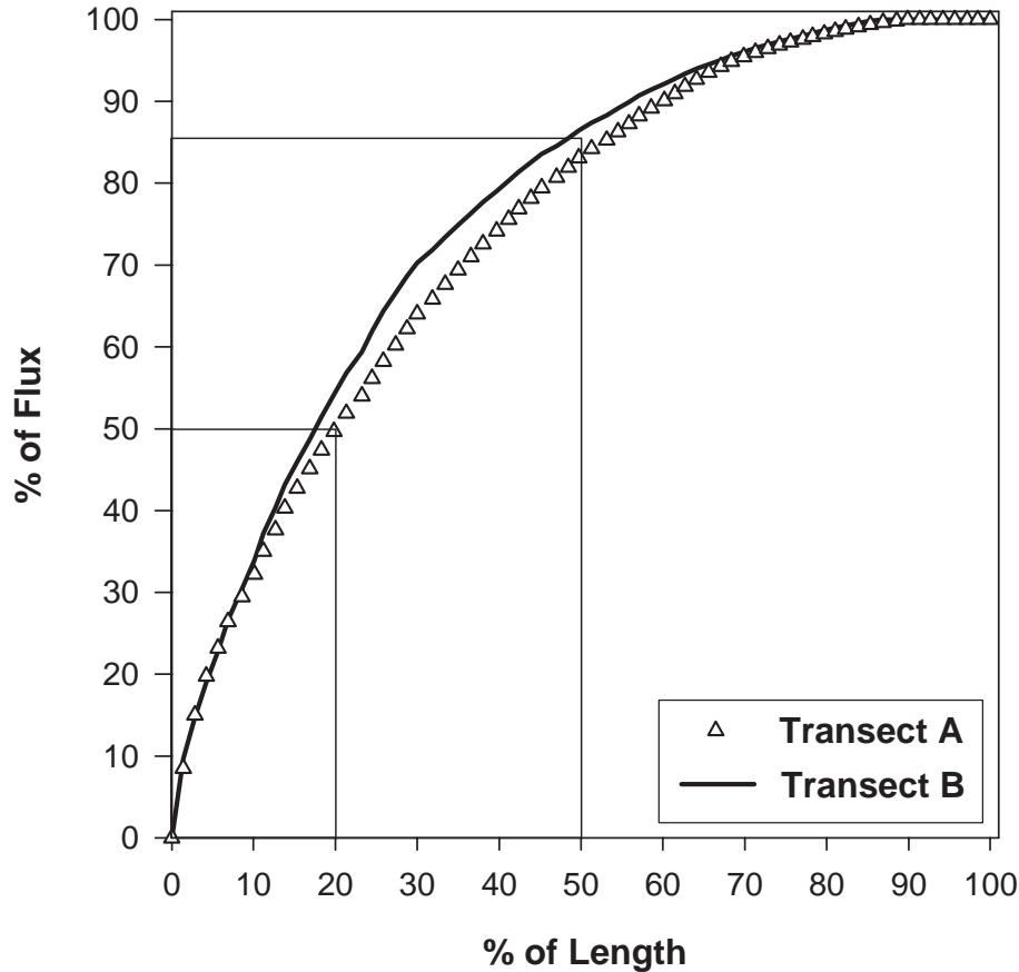
Fig. 7. Percentage of flux vs. percentage of length of the Transects A and B. Approximately 50% of the total flux occur on 20% of the total length.
