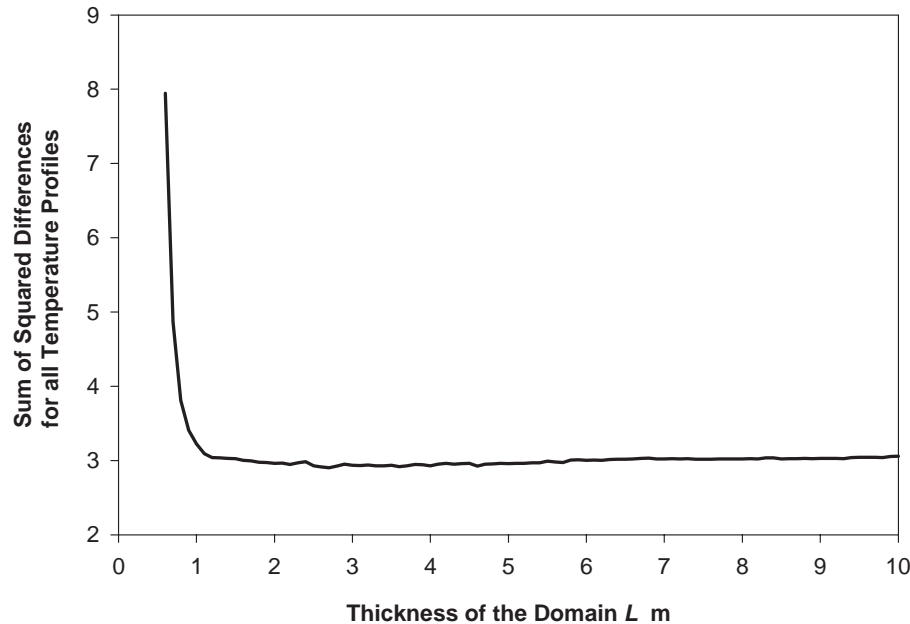
Fig. 5. Sum of squared errors of all temperature profiles vs. the length of the domain L . The results show that for the given parameter set, the quality of fit and the derived vertical fluxes are essentially constant for L > 1.0 m.
