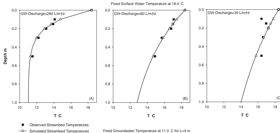
Fig. 6. Comparison of observed and simulated streambed temperatures for three example profiles. The illustrated profiles represent high (a), medium (b) and low (c) groundwater discharges and are located proximal to the positions of streambed piezometers P5 (a), P4 (b) and P1 (c).
