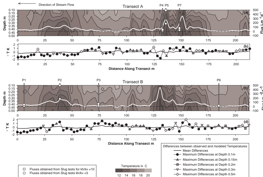
Fig. 4. Temperature distribution and temperature based fluxes and the locations of streambed piezometers and the fluxes from Darcy’s law calculations at each piezometer for different anisotropy ratios along Transects A (a) and B (c): Mean and maximum differences between observed and simulated temperatures for each temperature profile for Transects A (b) and B (d) The maximum difference is given with the respective depth.
