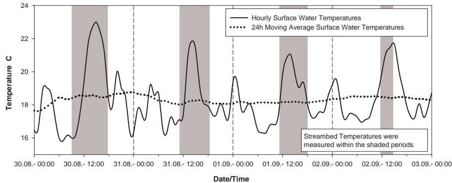
Fig. 3. Surface water temperatures during the four day measurement campaign in August/September 2005.
