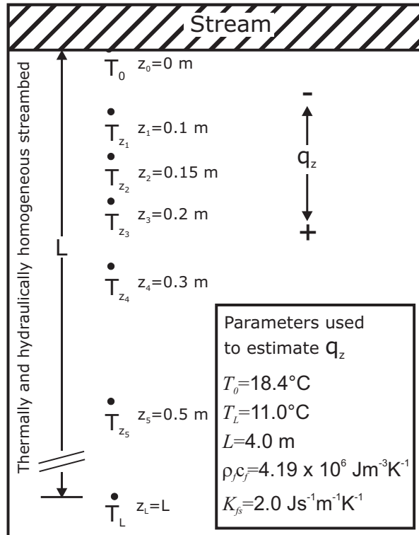
Fig. 2. Concept of vertical temperature profiles, boundary conditions and parameters used for the analytical model.
