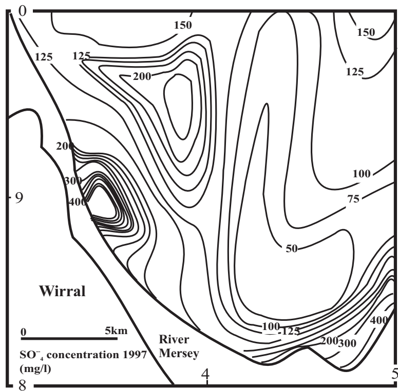
Fig. 5. Sulphate concentration (mg/l) in Merseyside UK for 1997.
