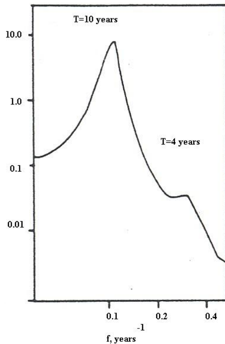
Fig. 11. The amplitude spectrum of the mean annual values of solar activity for the period 1950–1985.
