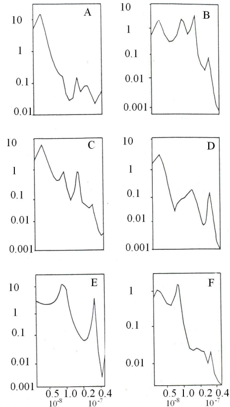
Fig. 7. Spectral characteristics of monthly values of solar activity and water level of Lake Tchudskoye: (a) the amplitude spectrum of solar activity for May 1943–July 1953; (b) the amplitude spectrum of the level of Lake Tchudskoye for May 1943–July 1953; (c) the cross amplitude spectrum for May 1943–July 1953; (d) the cross amplitude spectrum for July 1953–August 1963; (e) the cross amplitude spectrum for August 1963–August 1975; (f) the cross amplitude spectrum for August 1975–August 1985.
