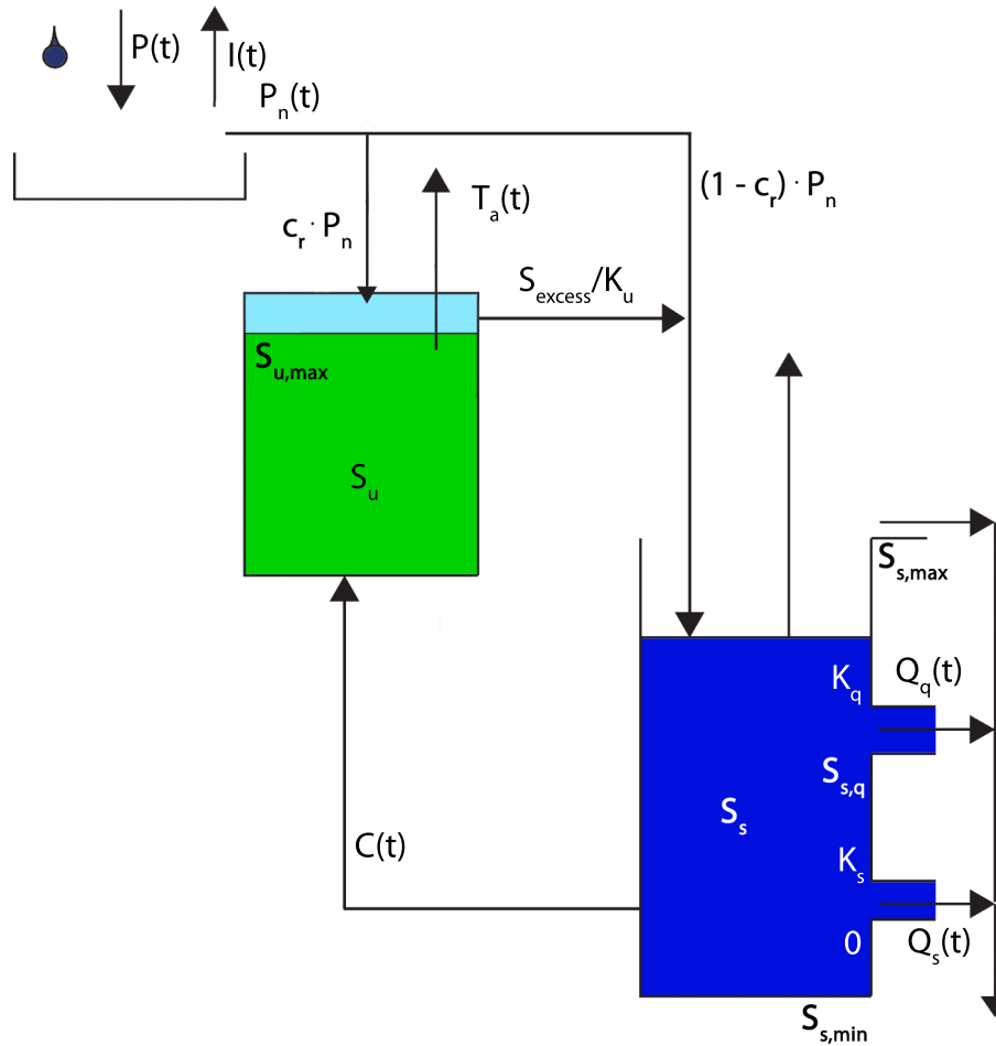
Fig. 6. STREAM conceptual model structure.
