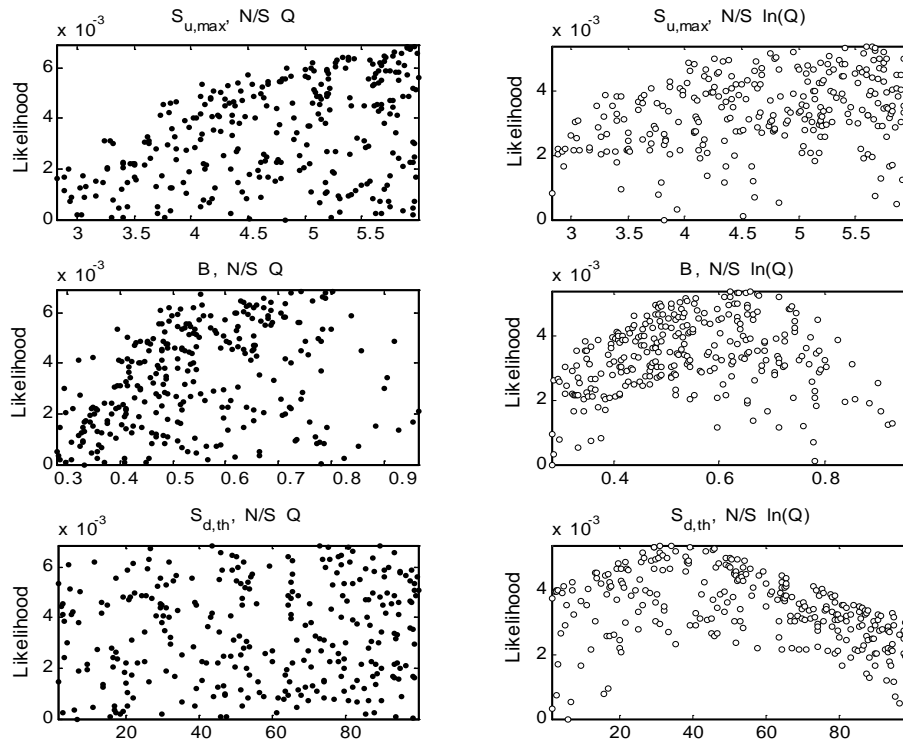
Fig. 9. GLUE likelihood dotty plots on Kabompo watershed. Filled dots: likelihoods for discharge. Open dots: likelihoods for the natural logarithmic of discharge. S_{u,max} [mm] is the maximum field capacity, B [-] is the power that describes the soil moisture capacity function and S_{d,th} [mm] is the drainage network threshold.
