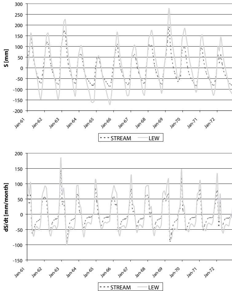
Fig. 12. Top: Estimated total storage. Bottom: Temporal change in total storage by STREAM and LEW.
