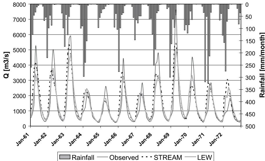
Fig. 11. Discharge time series at Victoria Falls from observations, STREAM and LEW results.
