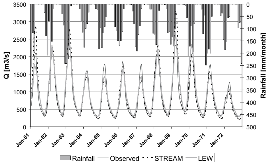
Fig. 10. Discharge time series at Lukulu from observations, STREAM and LEW results.
