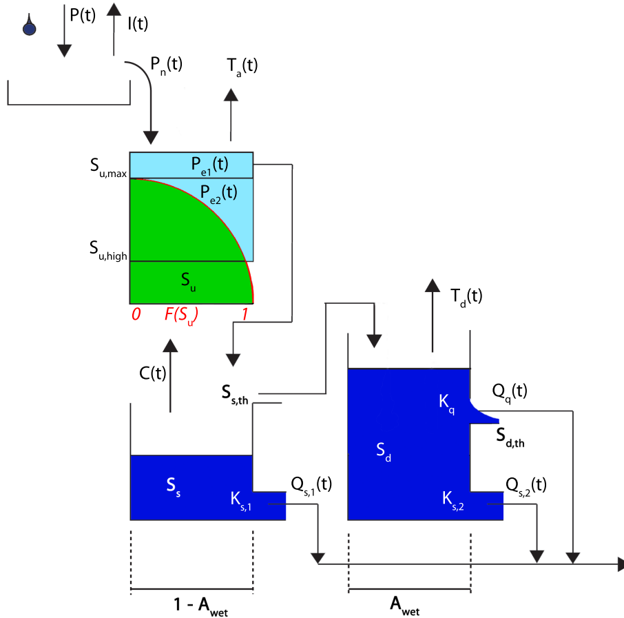
Fig. 8. LEW conceptual model structure.
