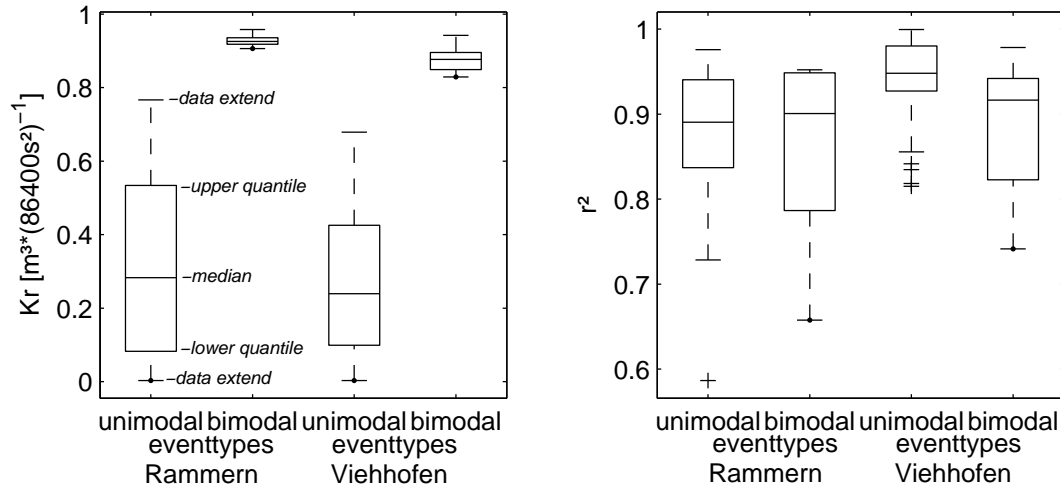
Fig. 10. Box plots of recession coefficients K_r (left) with goodness of curve fit r^2 (right) for the unimodal and bimodal event types at the small-catchment scale (gauge Rammern) and at the meso-scale (gauge Viehhofen).
