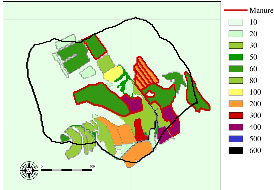
Fig. 2. Extraction coefficients map of the study watershed. Units: [\mu\text{g l}^{-1}] . Regularly manured areas outlined in red. Watershed boundary outlined in black.
