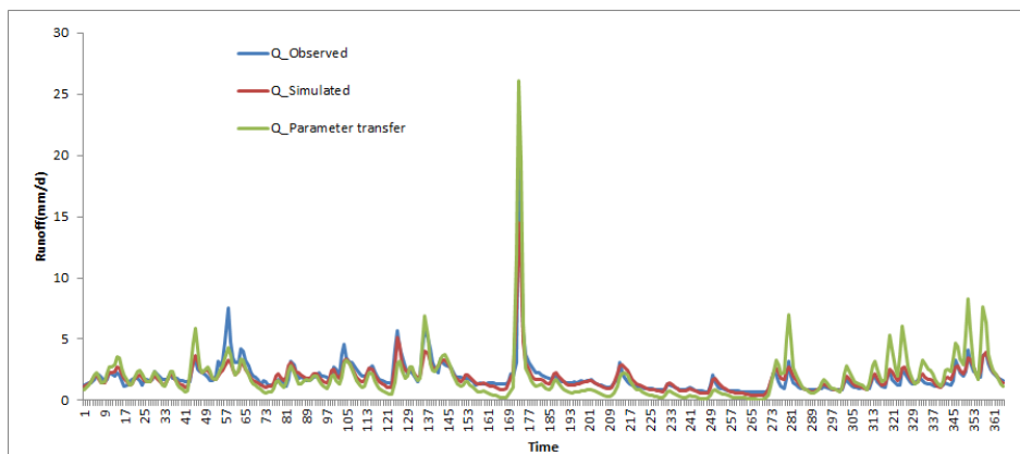
Fig. 2. Runoff hydrographs for catchment 12.
