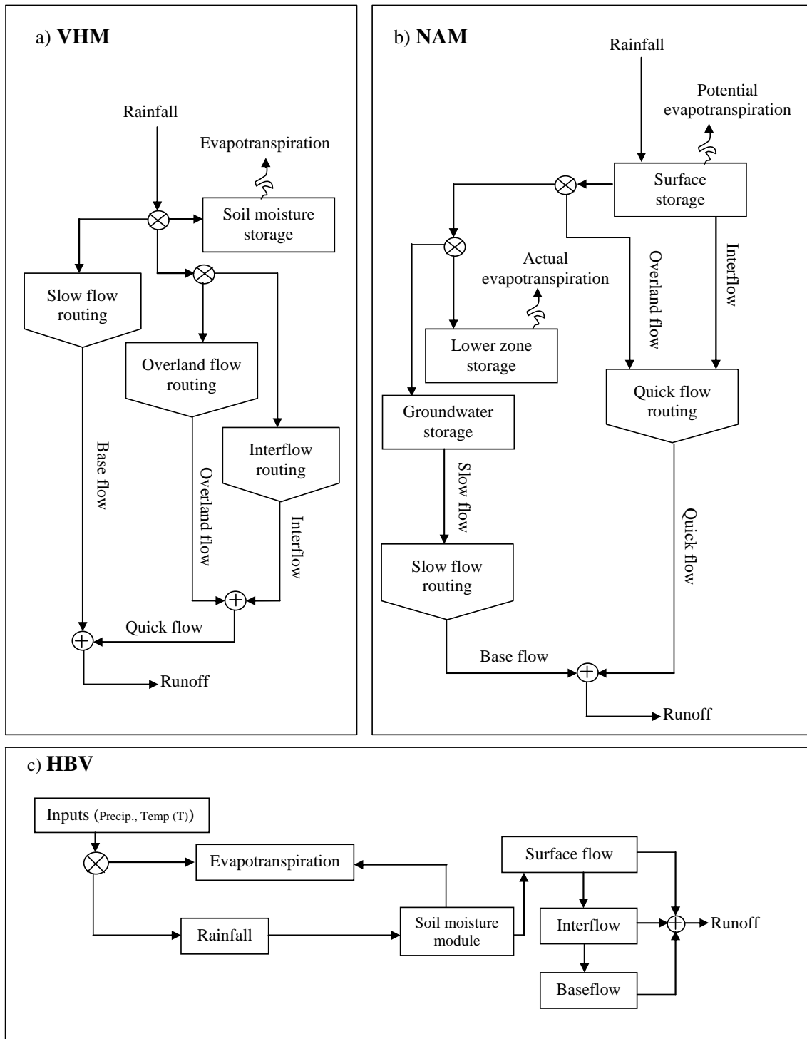
Figure 1 General processes of a) VHM, b) NAM, and c) HBV.
