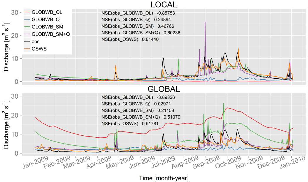
Figure 8. Simulated and observed streamflow estimates at 410088 gauging station in a tributary of the Murrumbidgee river for the time period January 2009-January 2010. The upper panel shows streamflow when local data is used as model forcing. Streamflow obtained with the global forced models is shown in the lower panel. Each panel contains results for each data assimilation scenario and the observed streamflow estimates plotted with different colours lines (OSWS — orange, GLOBWB_OL — red, GLOBWB_Q — blue, GLOBWB_SM — green, GLOBWB_SM+Q — purple and obs — black). The ensemble mean is given for each data assimilation scenario.
