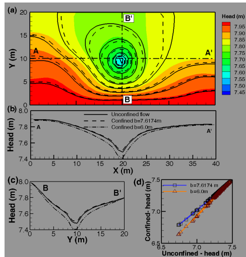
Figure 1. The comparison of head observations for unconfined and confined aquifers: (a) the plane view of the head distributions, (b) the head profiles along Y=10 m, (c) the head profiles along X=20 m, and (d) the scatterplot for head observations at well locations.
