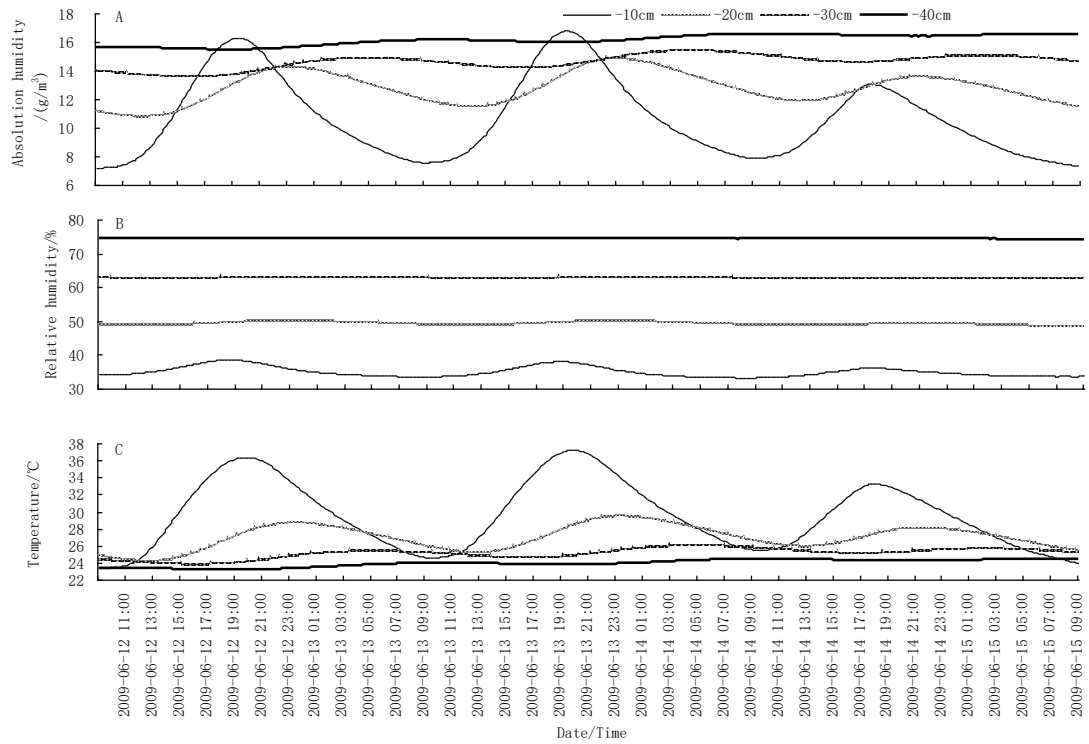
Fig. 4. Temperature and humidity at different soil depths in the greenhouse.
