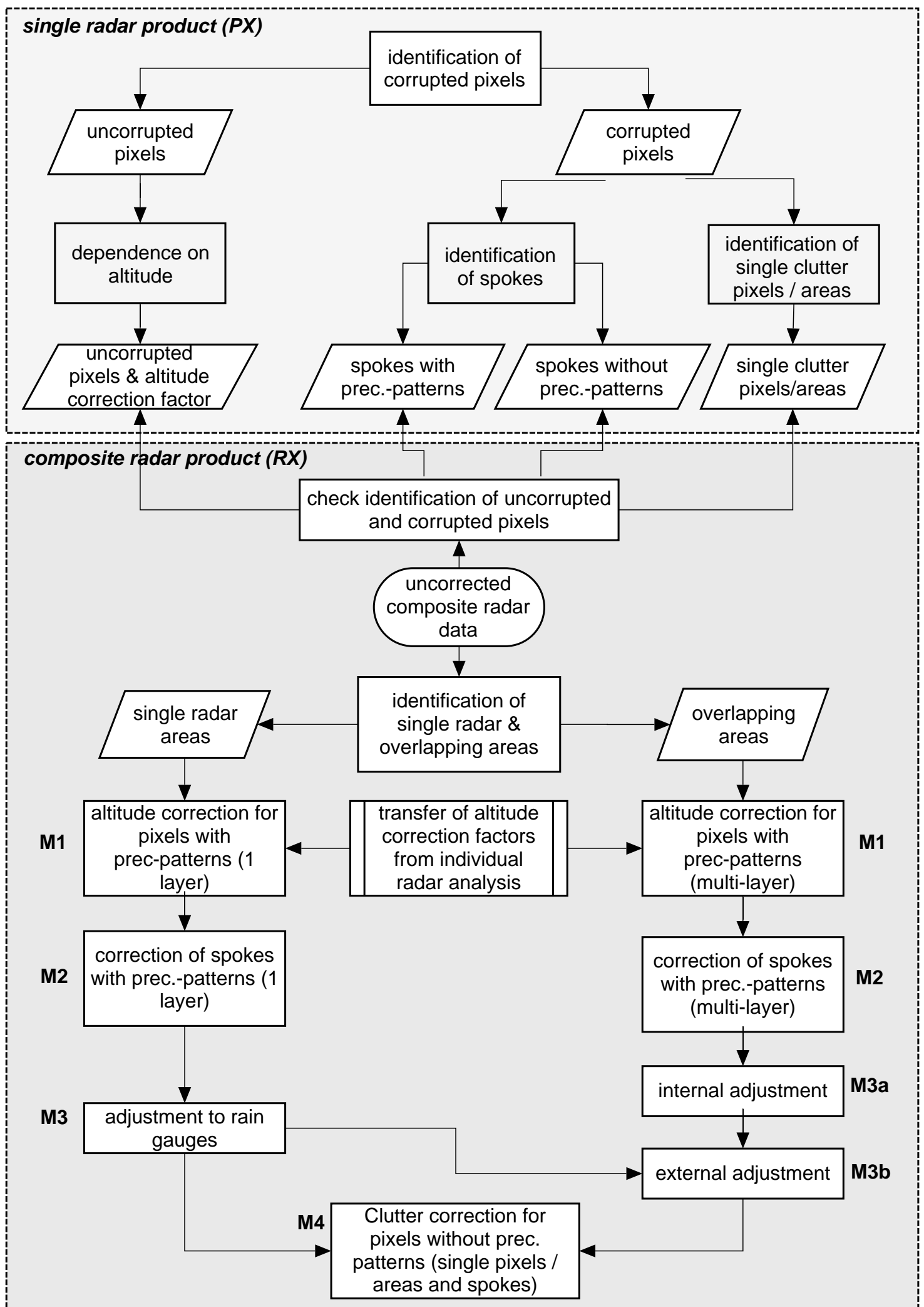
Fig.: Flowchart of the complete post-correction scheme. The modules are labelled M1 .. M4.
