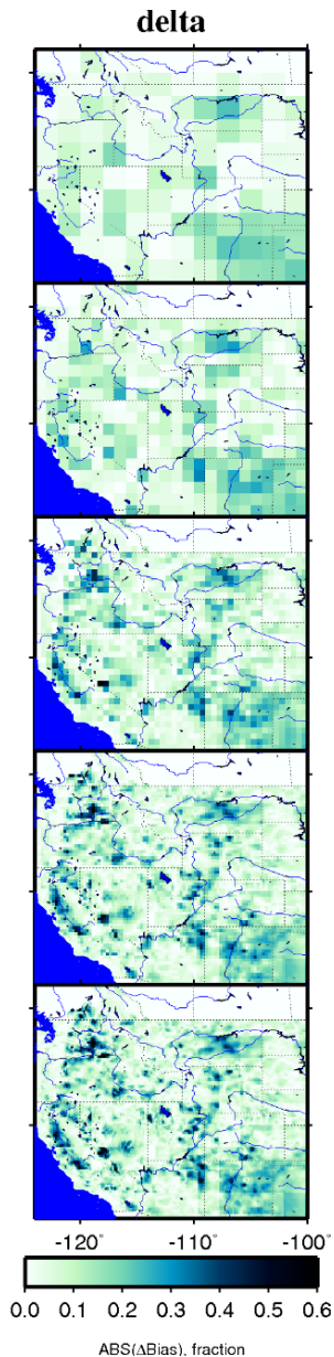
Figure 1 - The change in bias in mean daily precipitation between the calibration and validation period, expressed as an absolute fraction.
