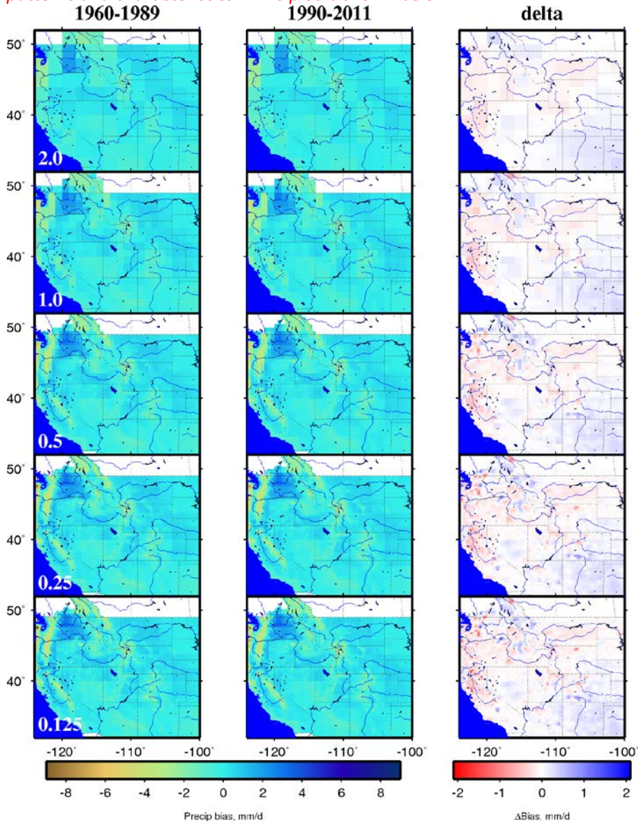
Figure 2 - Bias in mean annual maximum daily precipitation. This is comparable to Figure 3 in the Discussion paper, but for an extreme precipitation measure.
