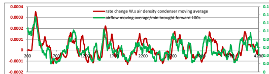
Fig. 2. The same as above, but with the air density change kinetic energy instead of the partial pressure change. The curves of the partial pressure change and the air density change of the same parcel of air are similar, with the difference in the quantities involved. The left-hand Y-axis gives the units in Watt.seconds and we see a 2000-fold difference between the two.
